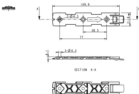
Mounting bracket (frame flat) w/M4 nuts - article No. 1015W1009:
