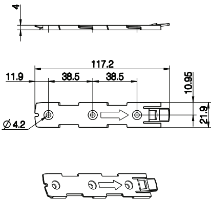
Mounting bracket (frame flat) - article No. 1015W1001:
