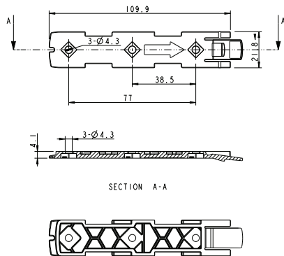
Mounting bracket (frame flat) w/M4 nuts - article No. 1015W1009:
