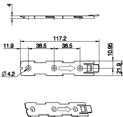
Mounting bracket (frame flat) - article No. 1015W1001:
