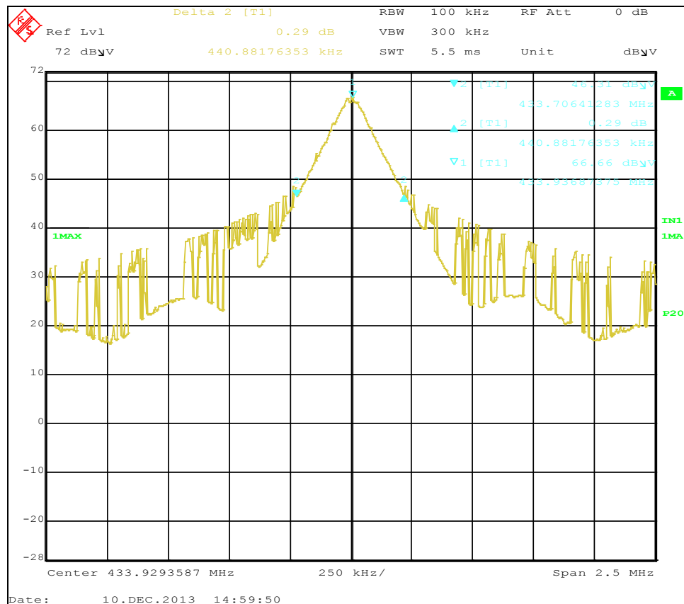
Plot 8. 20 dB Bandwidth Plot
