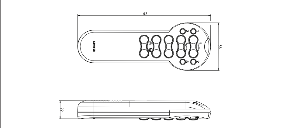
HC20RF Hand Control
