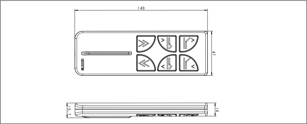
HB20RF Hand Control
