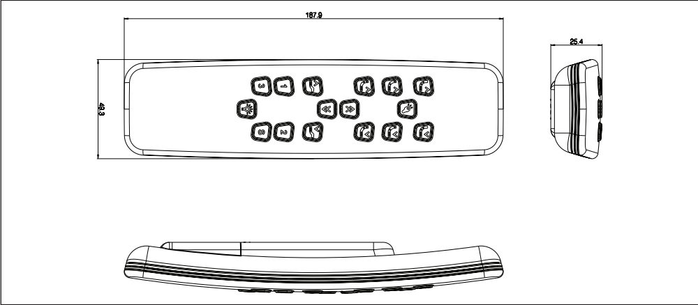
HC20RF Hand Control
