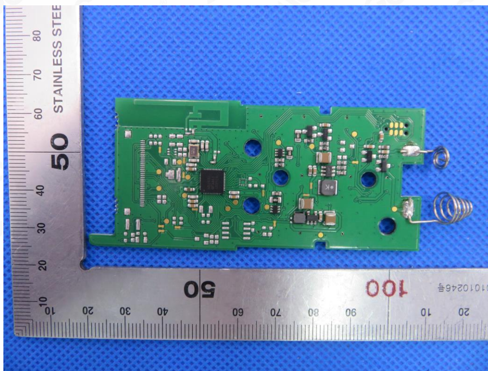
Fig.20 -main board view (type: HC42BL00S000000)
