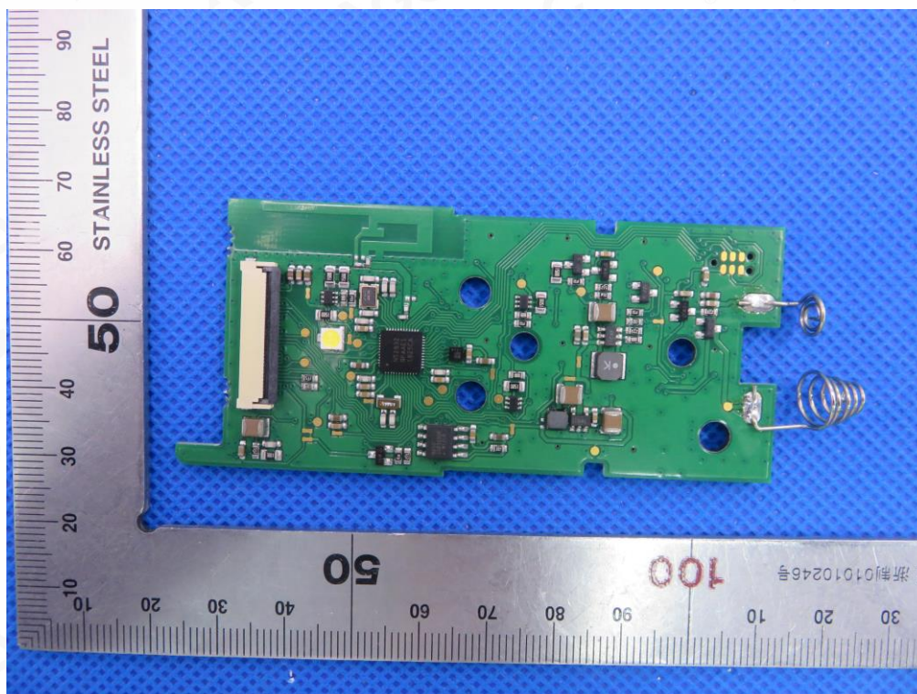
Fig.32-main board view (type: HC42BL01S000100)
