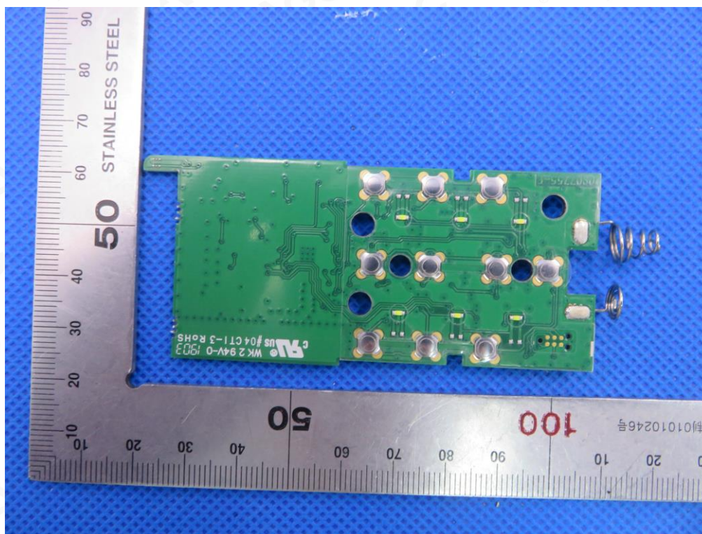
Fig.44 -main board view (type: HC42BL10S000000)
