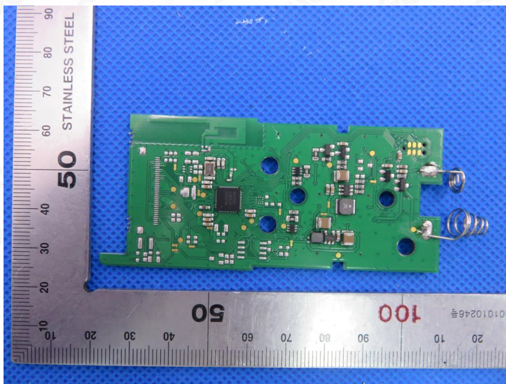
Fig.42 -main board view (type: HC42BL10S000000)
