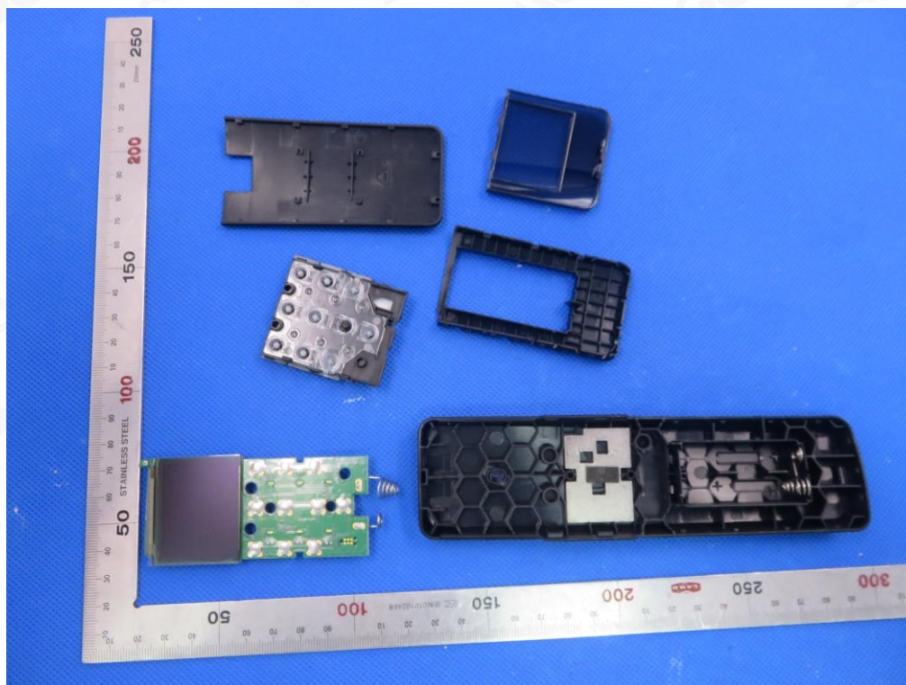
Fig.30 -internal view (type: HC42BL01S000100)
