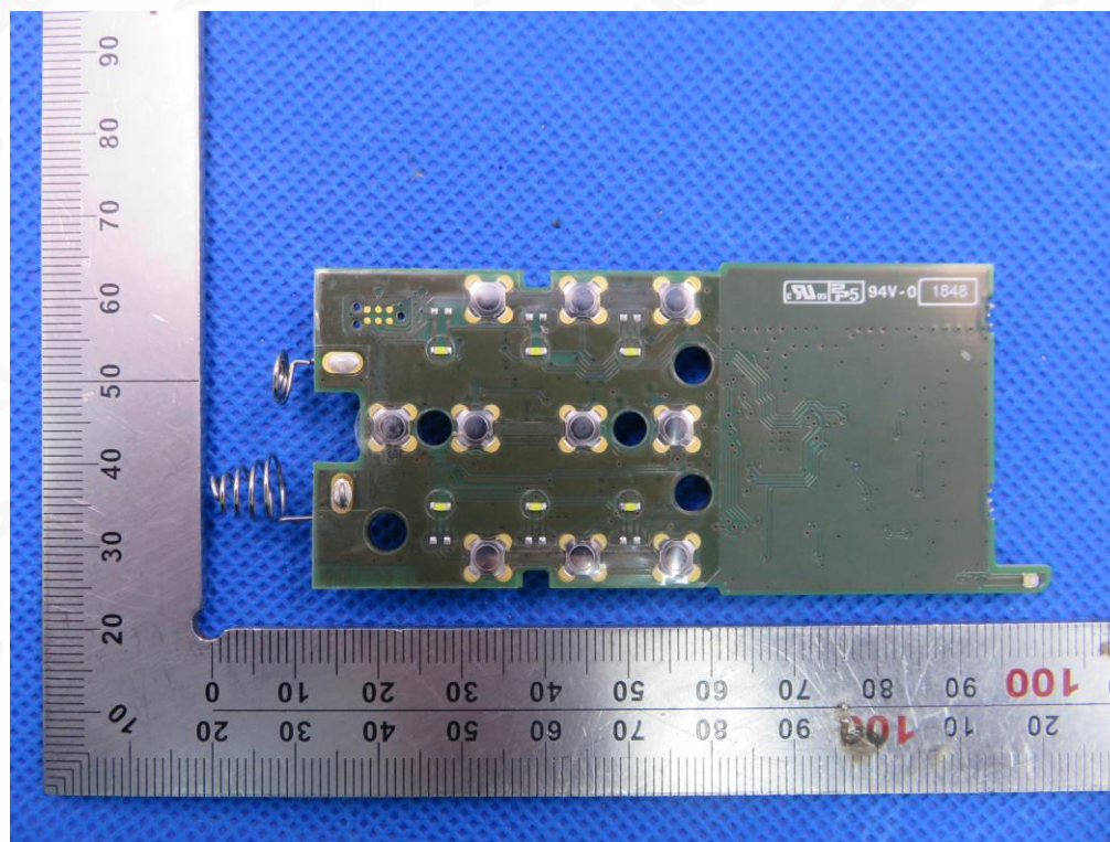
Fig.10 -main board view (type: HC42BL11S000100)
