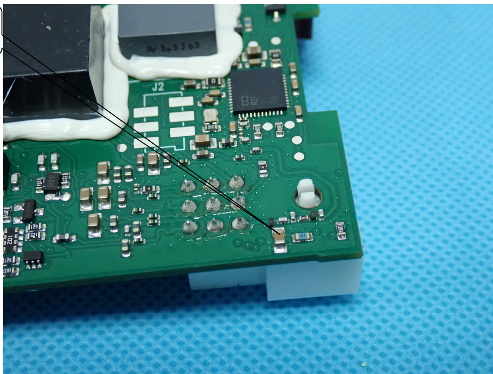
Internal Photo 5
