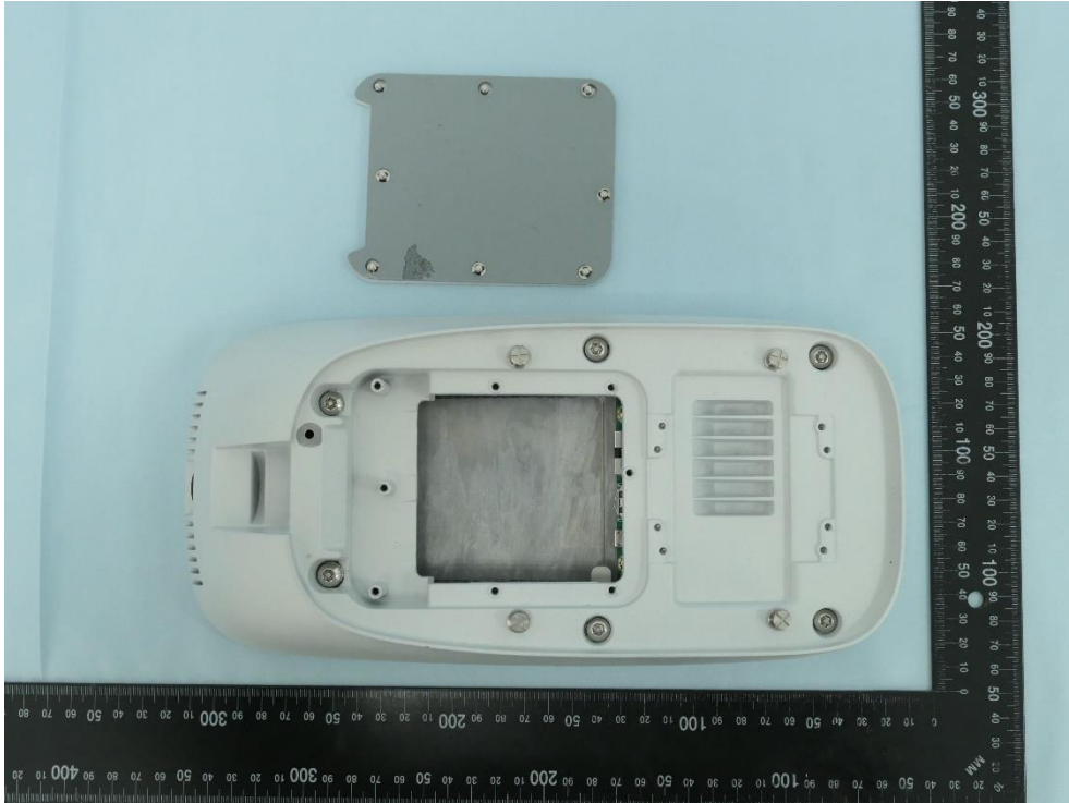
(7) EUT Photo
