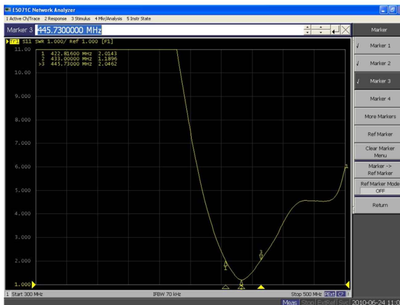
23 MHz Bandwidth Measurement (433 MHz) of @ SWR of 2.0
