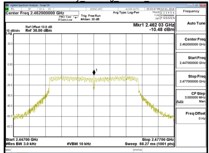
Power Density 802.11g Chain0 2462MHz
