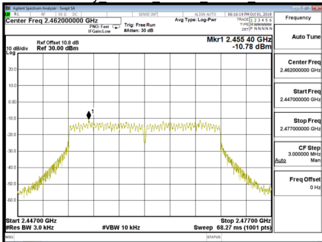
Power Density 802.11n 20MHz Chain0 2462MHz
