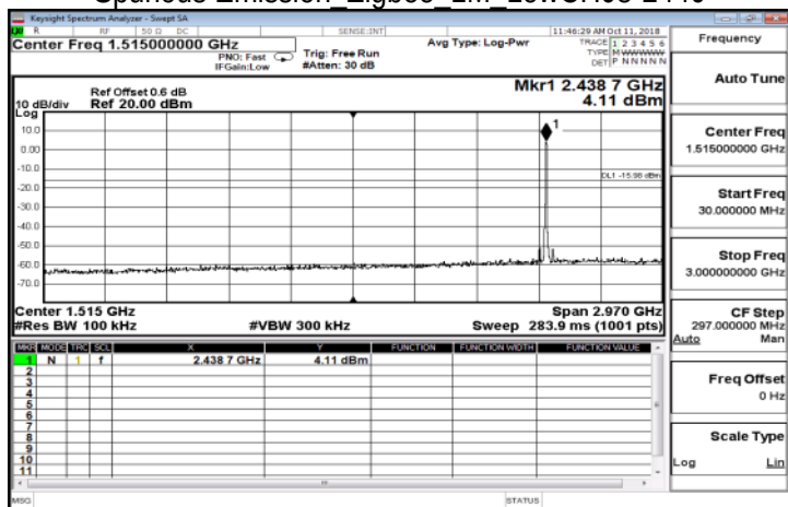
Spurious Emission Zigbee 1M LowCH08-2440
