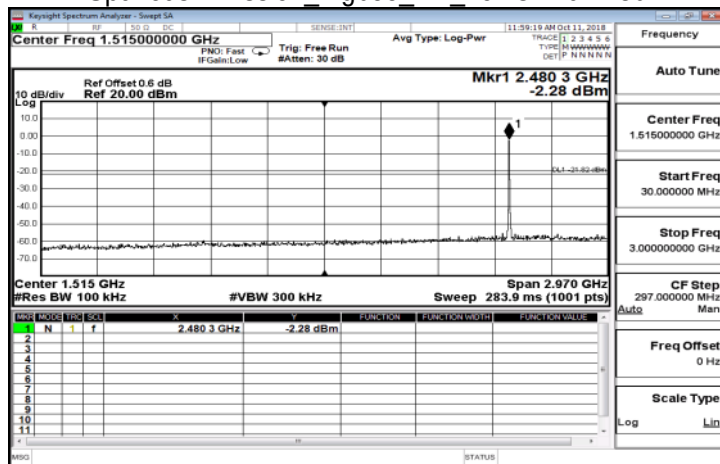
Spurious Emission Zigbee 1M HighCH16-2480
