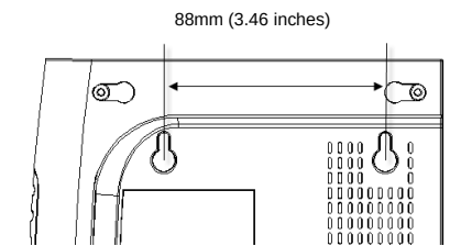
The Distance of the Pothook (Horizontal)
