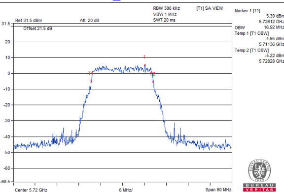
802.11a_Chain 3 / CH144
