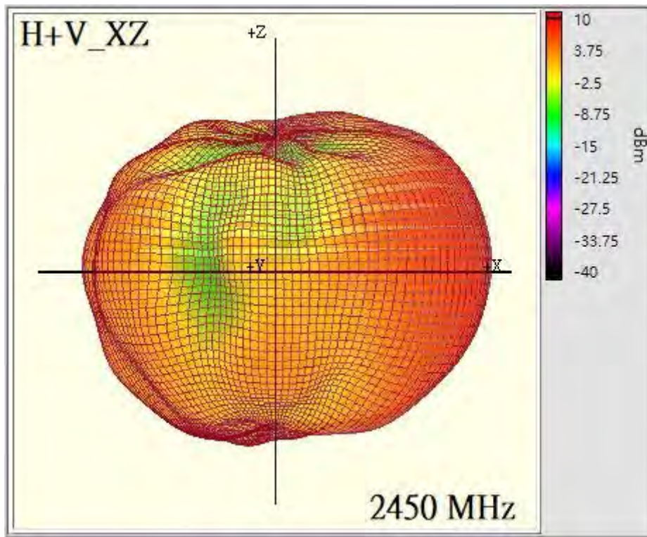
XZ Plan(2450MHz)
