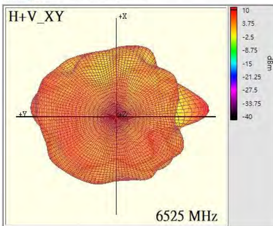
XY Plan(6525MHz)
