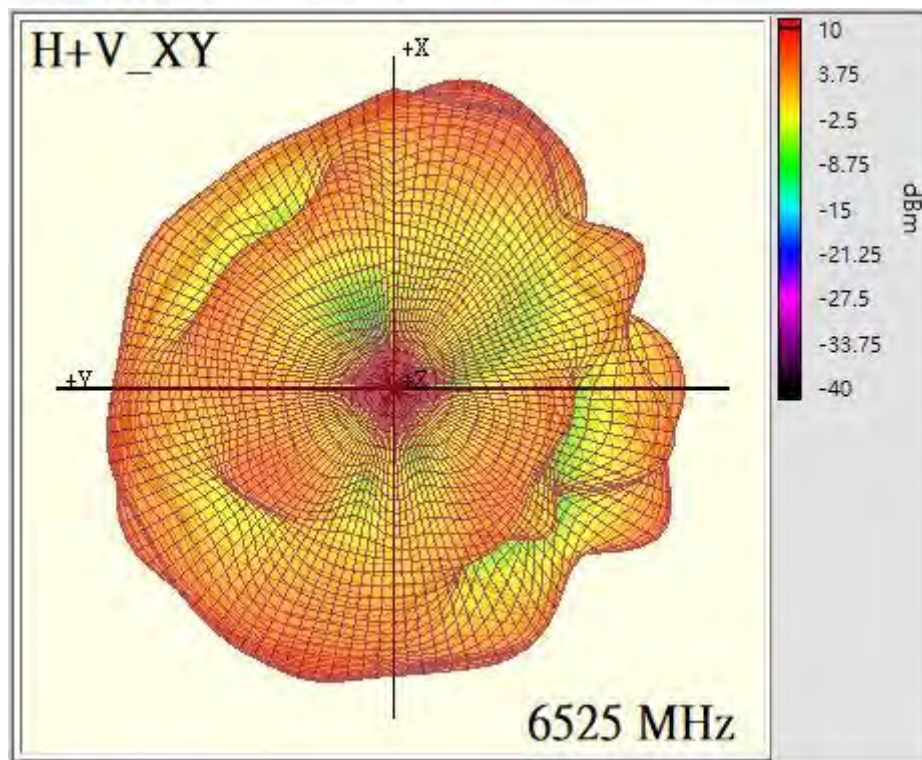
XY Plan(6525MHz)
