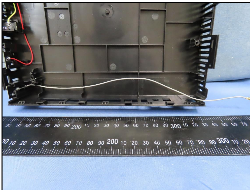
DB1 antenna
