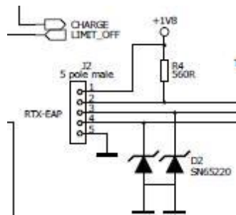
Figure 4: Debug connector
