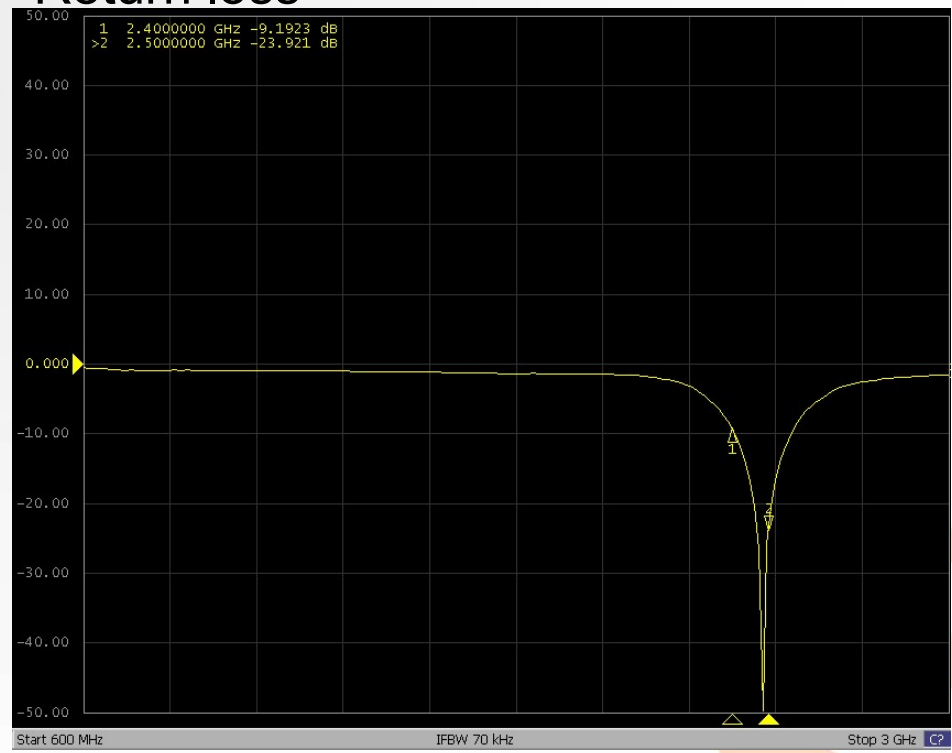
Return loss
