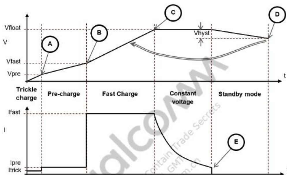
Figure 9-1 Charge cycle states
