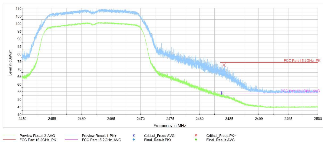
Fig.4 Transmitter Spurious Emission - Radiated (Power): 802.11g, ch11, 2.45 GHz - 2.50GHz
