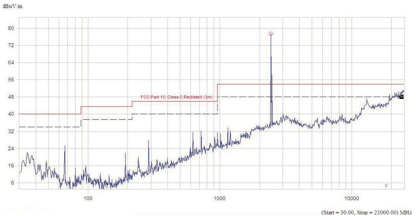
(Plot B.2: Antenna Vertical)
