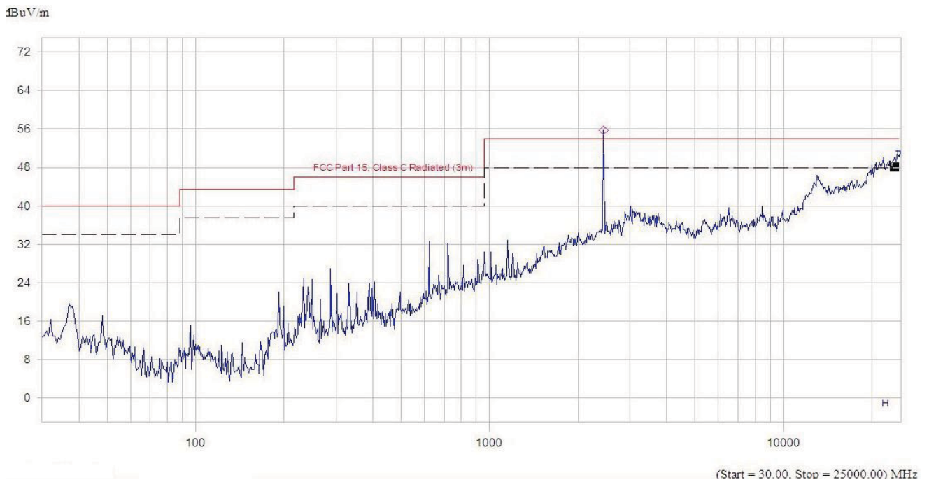
(Plot B.1: Antenna Horizontal)
