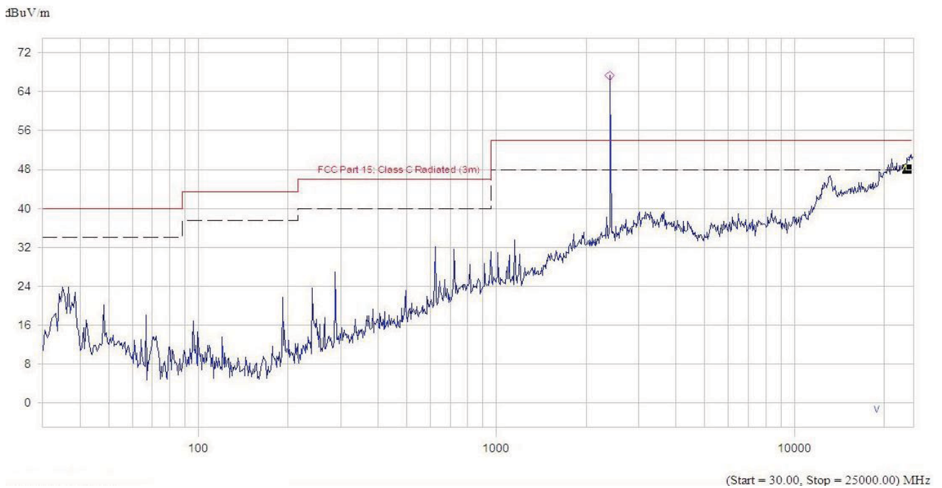
(Plot A.2: Antenna Verticalz)
