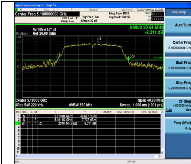
11a-Ant4-5180
