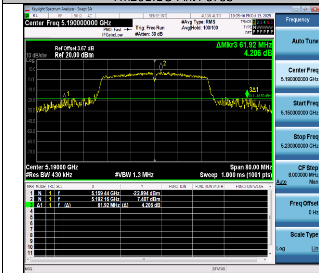
11n40SISO-Ant4-5190
