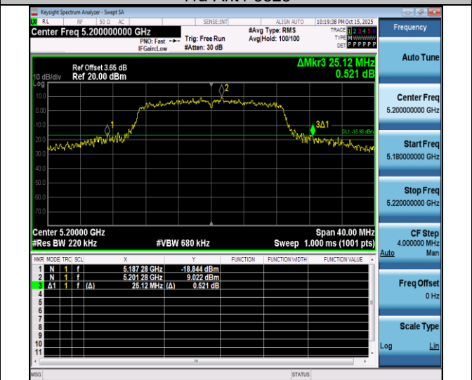
11n20SISO-Ant4-5200
