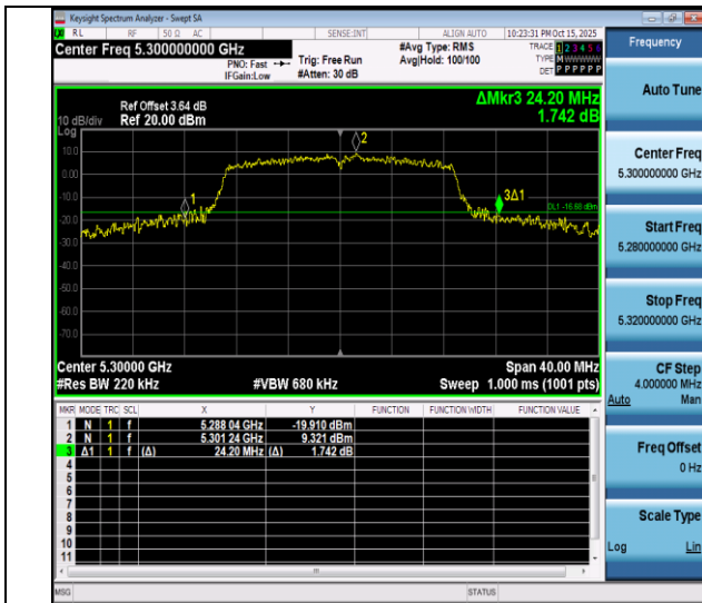
11n20SISO-Ant4-5300
