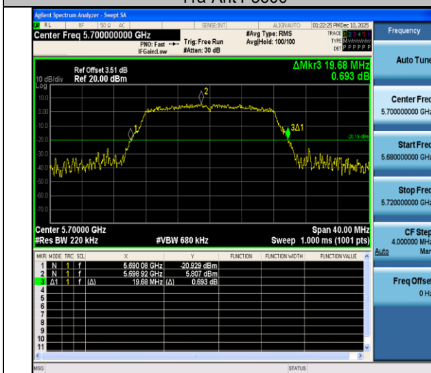
11a-Ant4-5700
