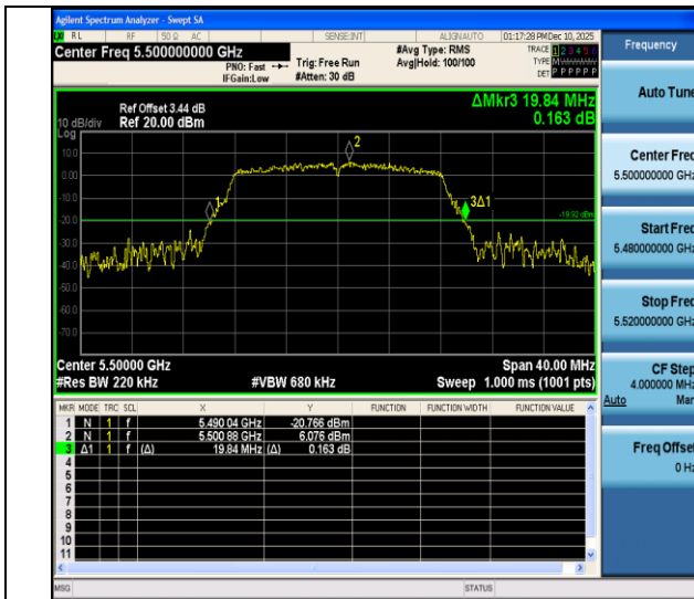
11a-Ant4-5500
