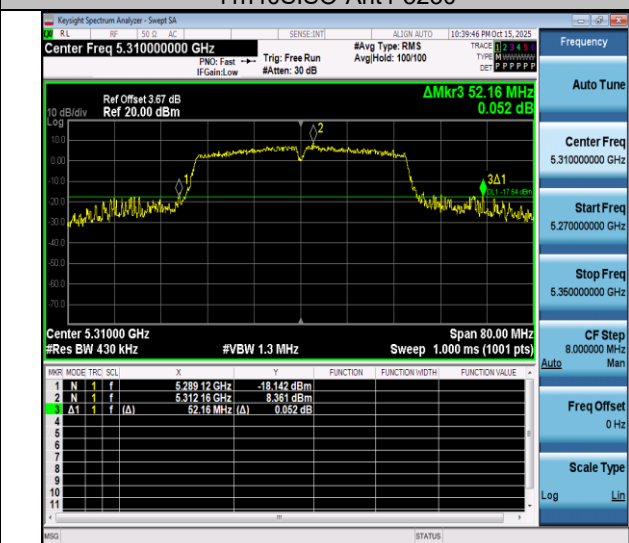
11n40SISO-Ant4-5310
