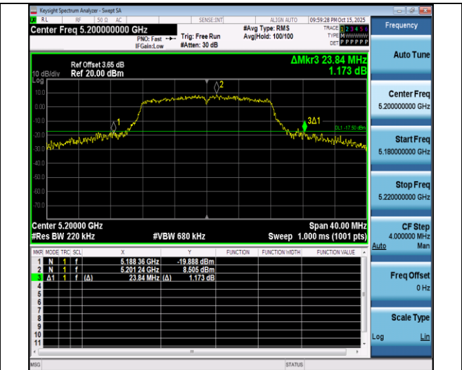
11a-Ant4-5200
