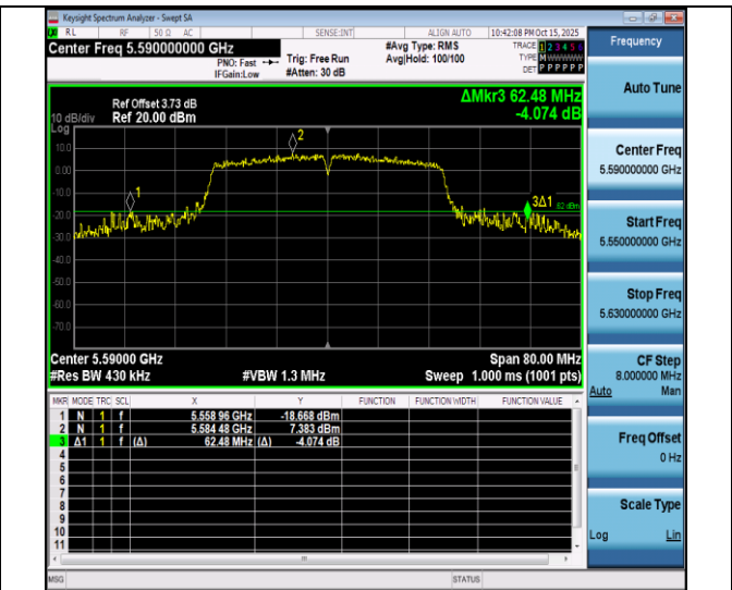
11n40SISO-Ant4-5590
