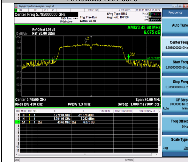
11n40SISO-Ant4-5795
