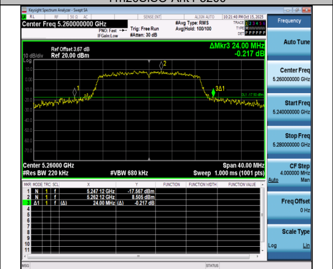
11n20SISO-Ant4-5260
