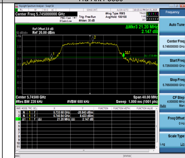
11a-Ant4-5745
