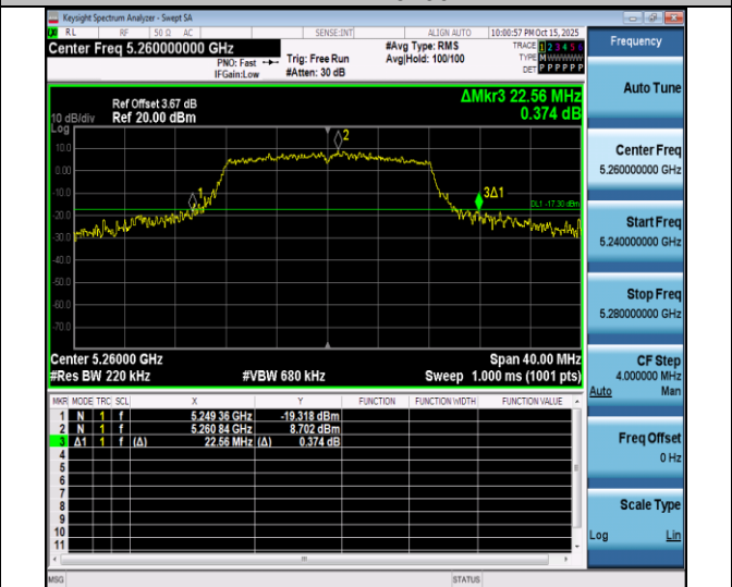
11a-Ant4-5260
