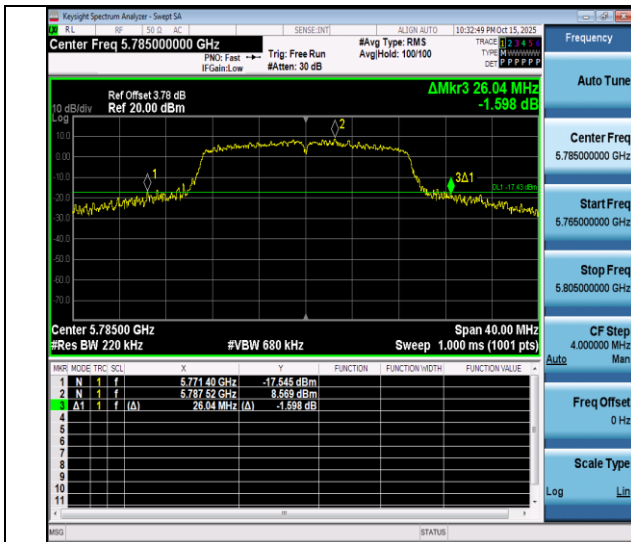
11n20SISO-Ant4-5785
