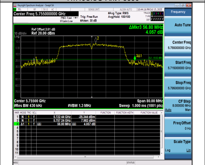
11n40SISO-Ant4-5755
