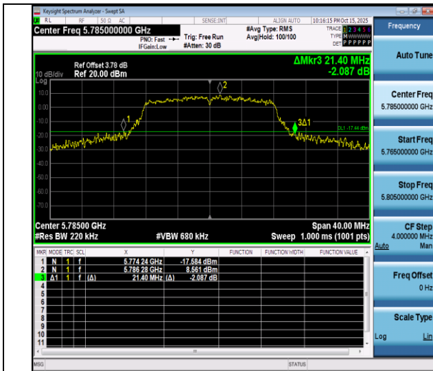
11a-Ant4-5785
