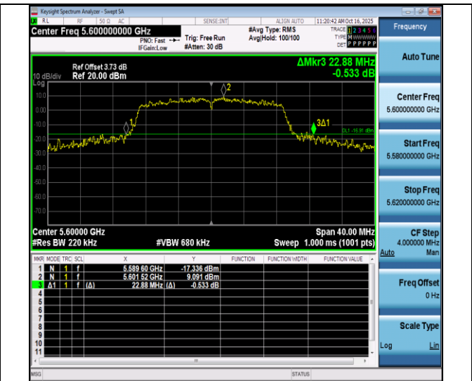
11ac20ISO-Ant4-5600
