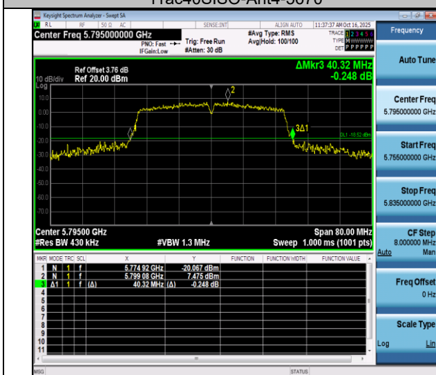
11ac40SISO-Ant4-5795
