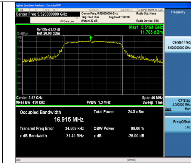
11a-Ant4-5520
