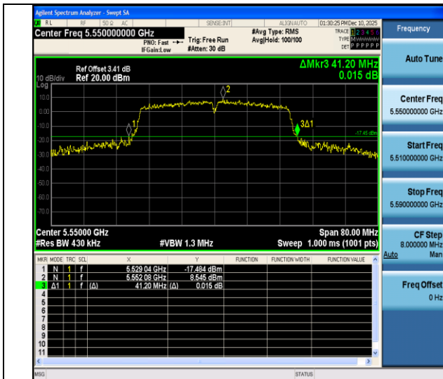
11ac40SISO-Ant4-5550
