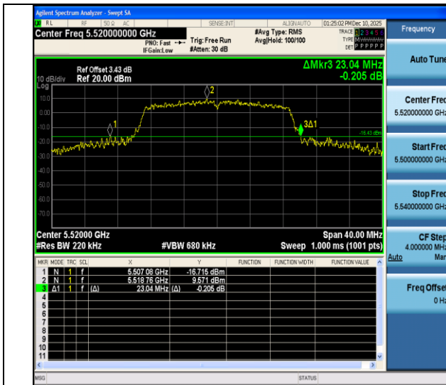
11ac20ISO-Ant4-5520
