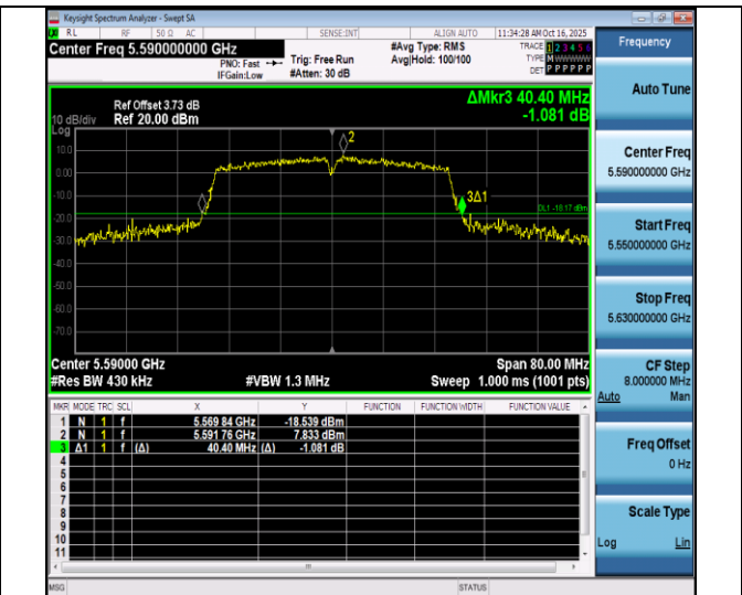
11ac40SISO-Ant4-5590
