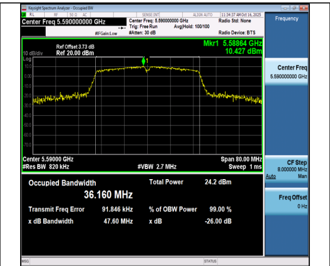
11ac40SISO-Ant4-5590
