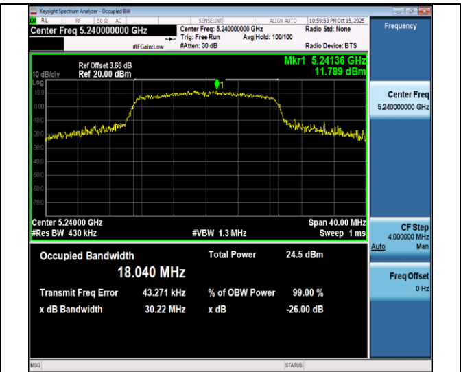
11ac20SISO-Ant4-5240
