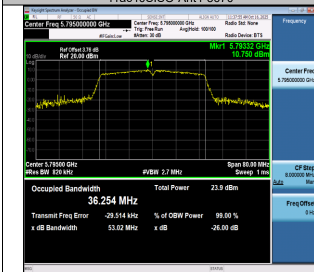
11ac40SISO-Ant4-5795
