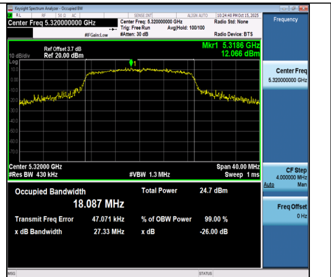
11n20SISO-Ant4-5320
