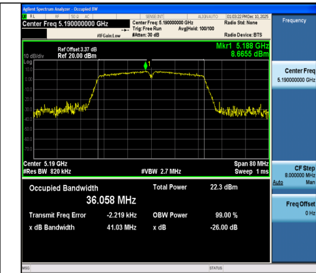
11ac40SISO-Ant4-5190
