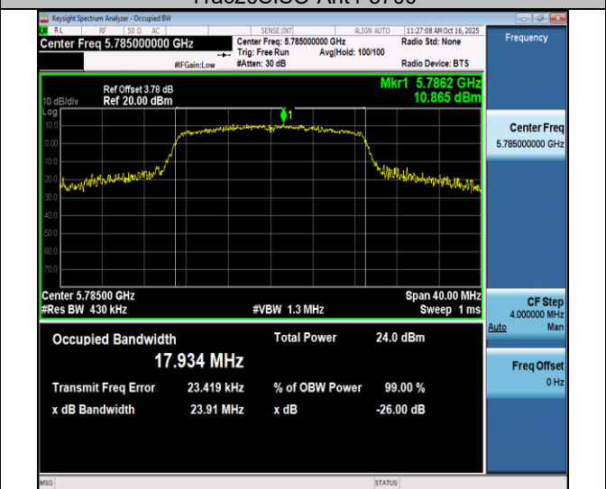
11ac20SISO-Ant4-5785
