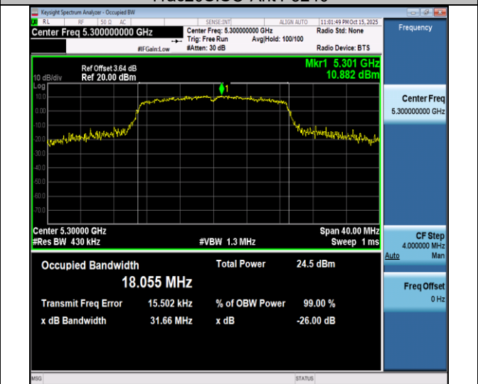
11ac20SISO-Ant4-5300
