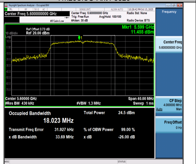
11n20SISO-Ant4-5600
