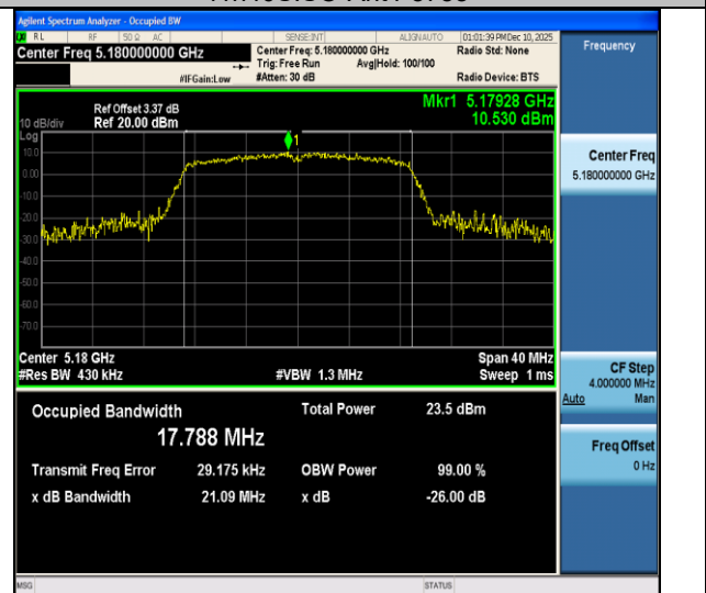
11ac20SISO-Ant4-5180
