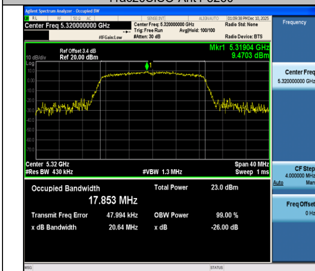
11ac20SISO-Ant4-5320
