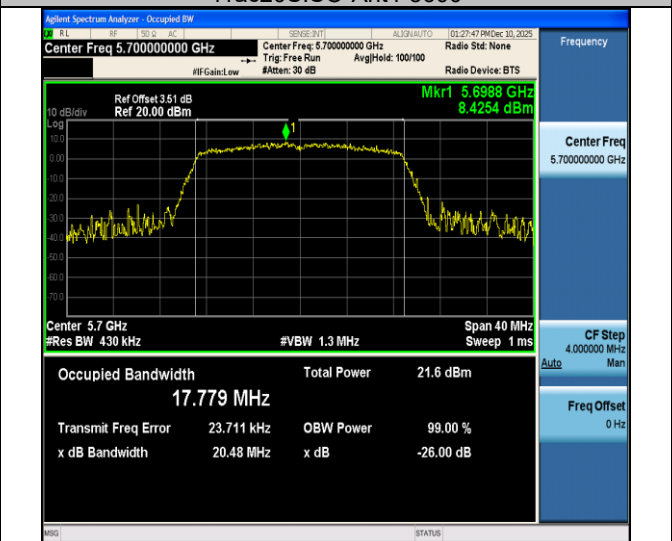
11ac20SISO-Ant4-5700
