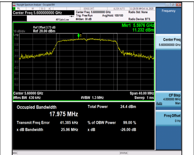
11ac20SISO-Ant4-5600
