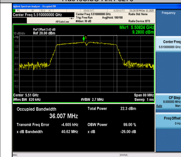
11ac40SISO-Ant4-5510
