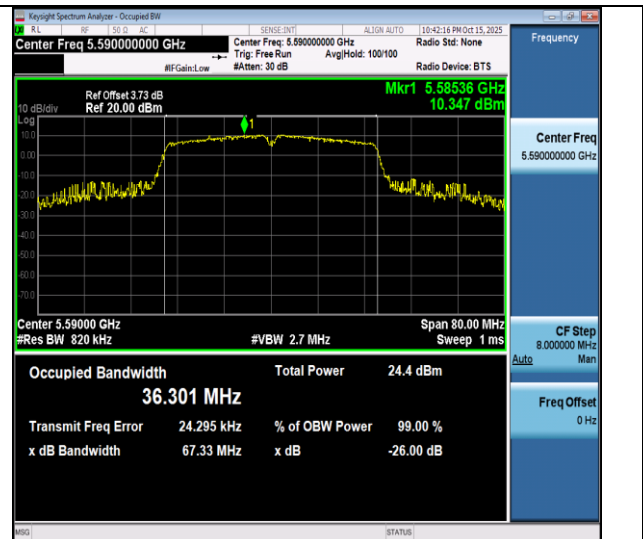
11n40SISO-Ant4-5590
