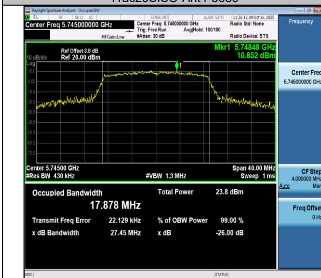
11ac20SISO-Ant4-5745
