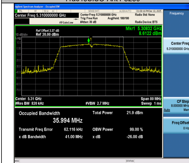
11ac40SISO-Ant4-5310
