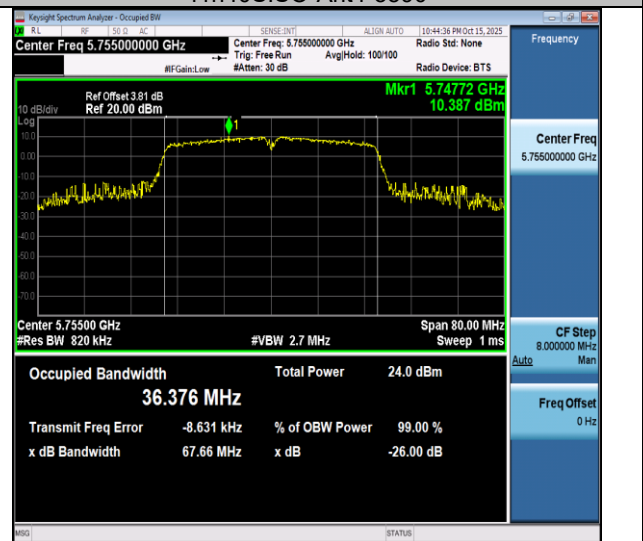
11n40SISO-Ant4-5755
