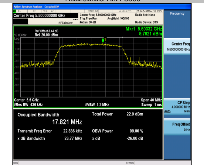
11ac20SISO-Ant4-5500
