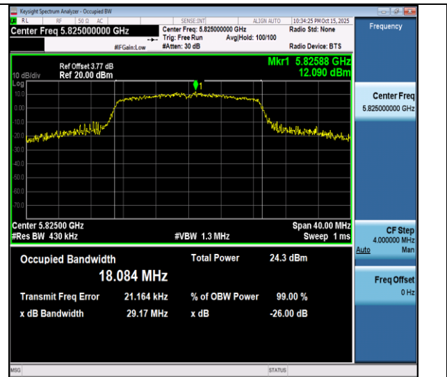
11n20SISO-Ant4-5825
