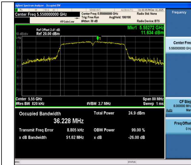
11ac40SISO-Ant4-5550
