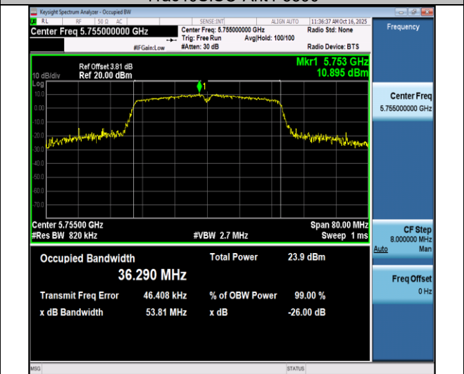
11ac40SISO-Ant4-5755
