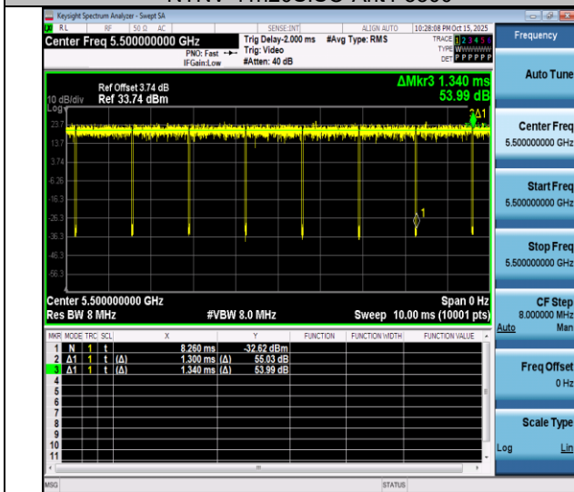
NTNV-11n20SISO-Ant4-5500
