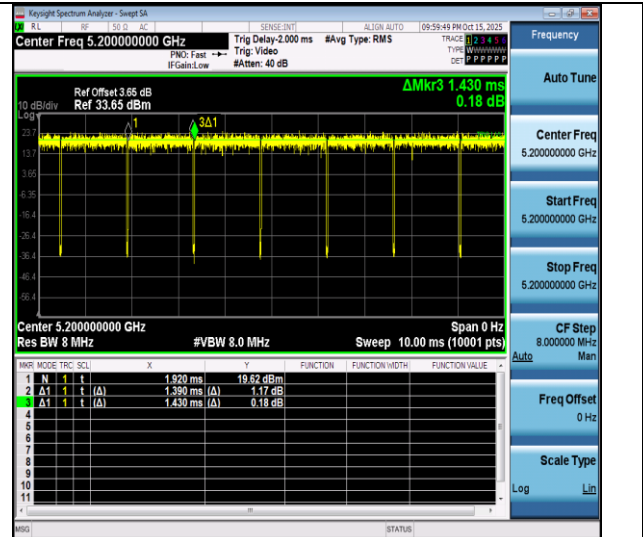
NTNV-11a-Ant4-5200
