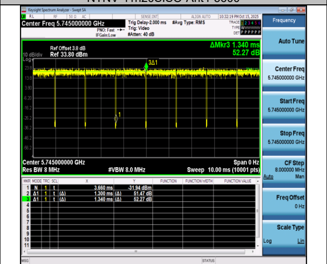
NTNV-11n20SISO-Ant4-5745
