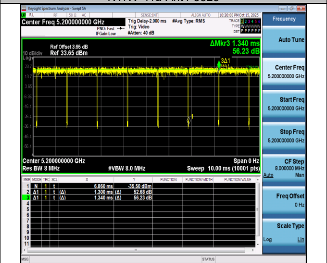
NTNV-11n20SISO-Ant4-5200
