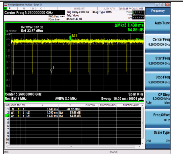
NTNV-11a-Ant4-5260
