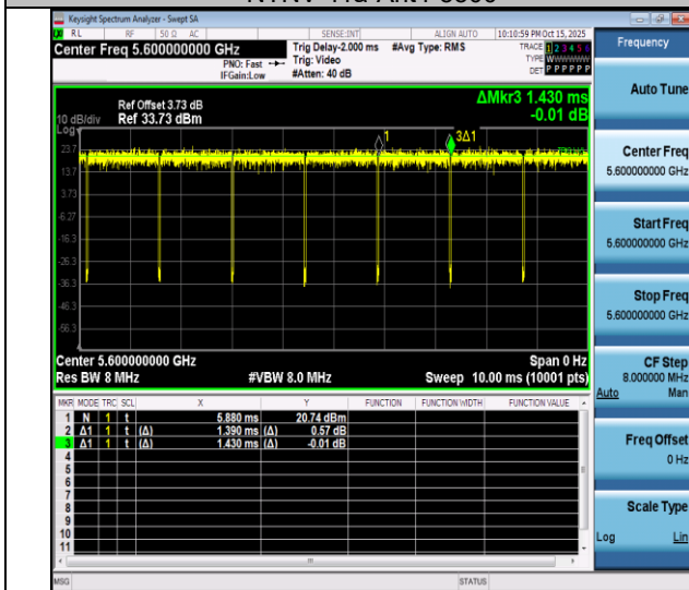
NTNV-11a-Ant4-5600
