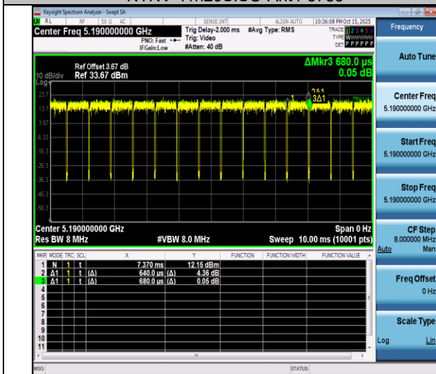
NTNV-11n40SISO-Ant4-5190
