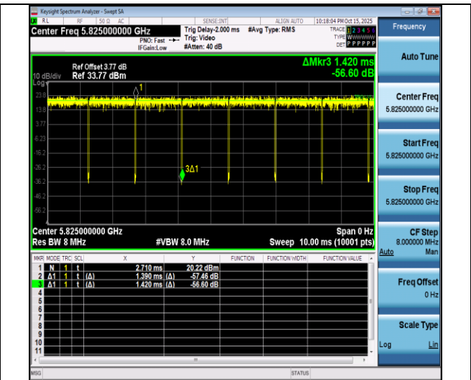
NTNV-11a-Ant4-5825
