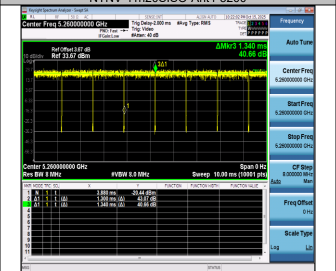
NTNV-11n20SISO-Ant4-5260
