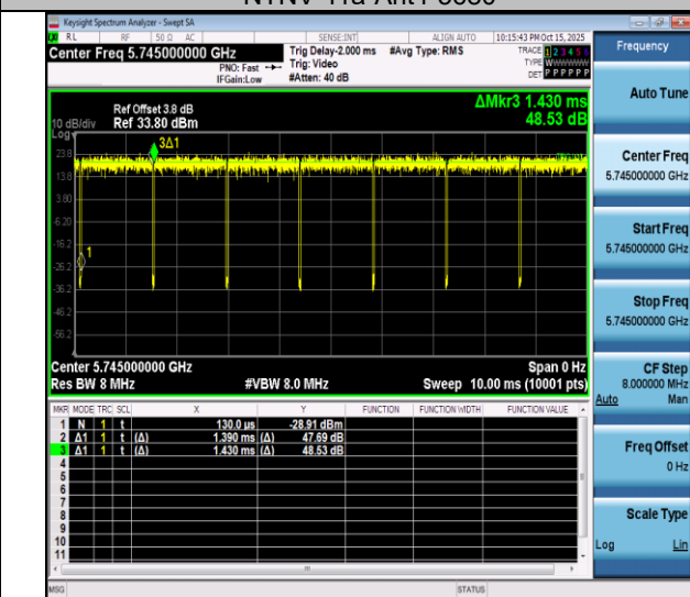
NTNV-11a-Ant4-5745
