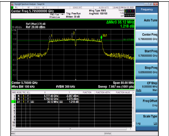
11n40SISO-Ant4-5795-PASS
