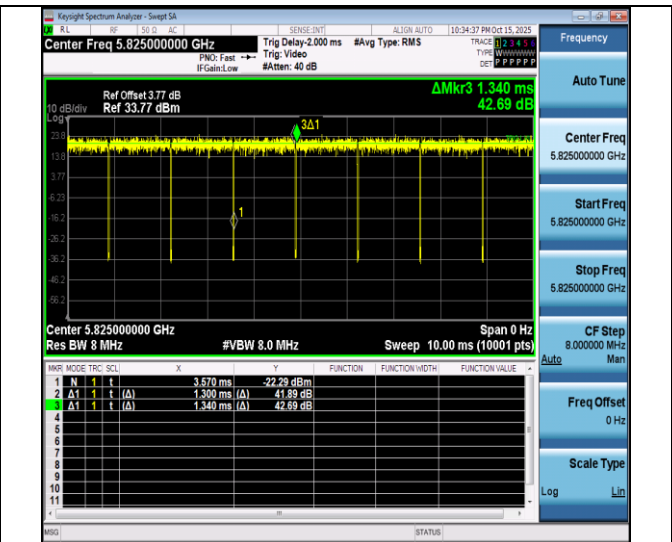
NTNV-11n20SISO-Ant4-5825
