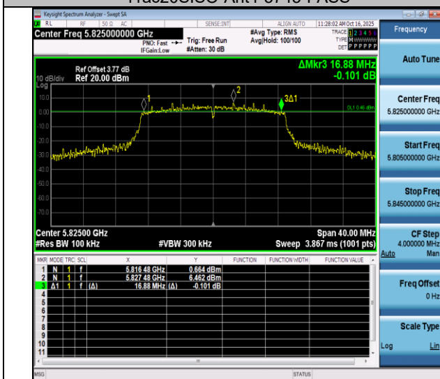
11ac20SISO-Ant4-5825-PASS
