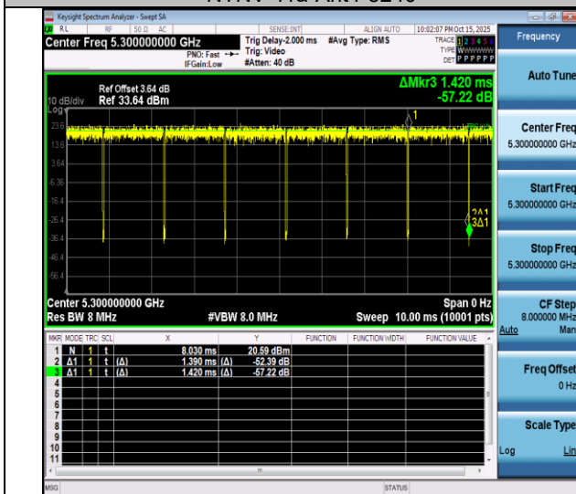
NTNV-11a-Ant4-5300
