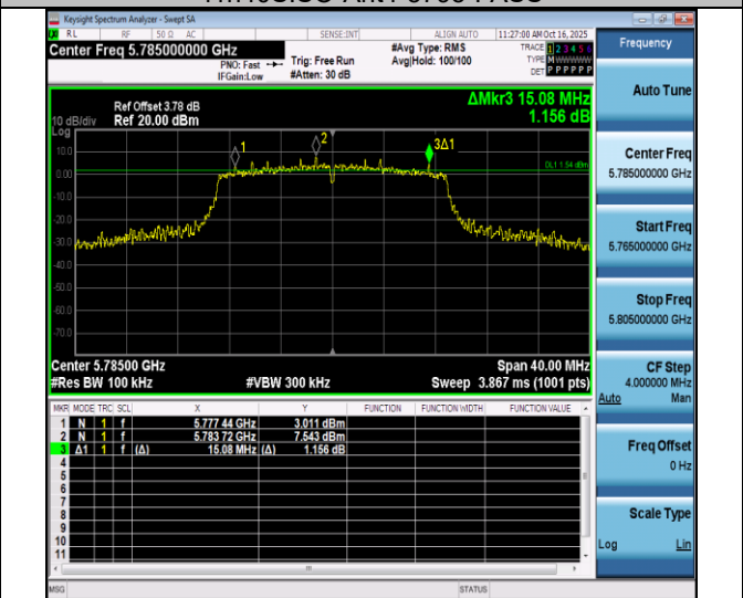
11ac20SISO-Ant4-5785-PASS
