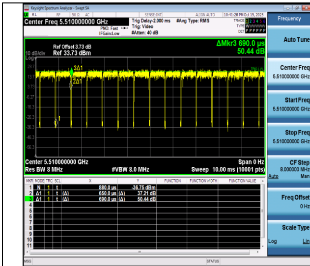
NTNV-11n40SISO-Ant4-5510
