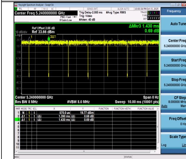
NTNV-11a-Ant4-5240
