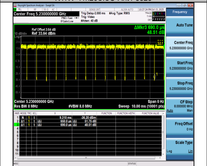
NTNV-11n40SISO-Ant4-5230
