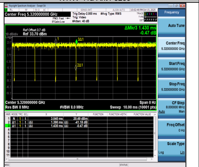
NTNV-11a-Ant4-5320
