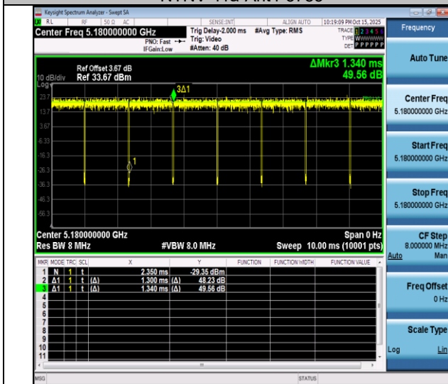
NTNV-11n20SISO-Ant4-5180
