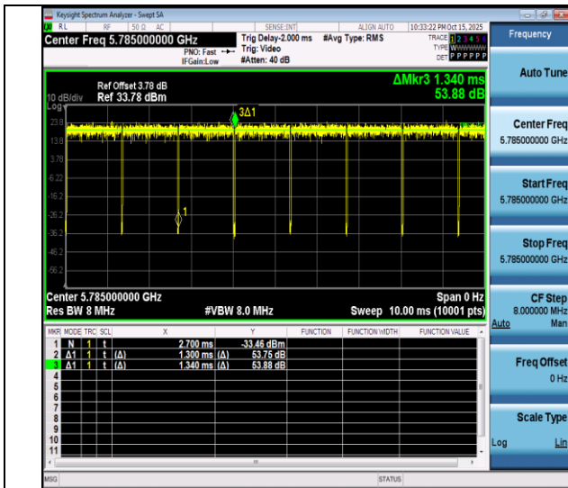
NTNV-11n20SISO-Ant4-5785
