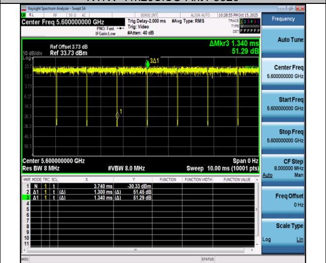
NTNV-11n20SISO-Ant4-5600
