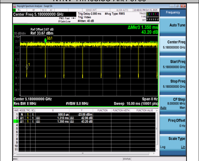
NTNV-11ac20SISO-Ant4-5180
