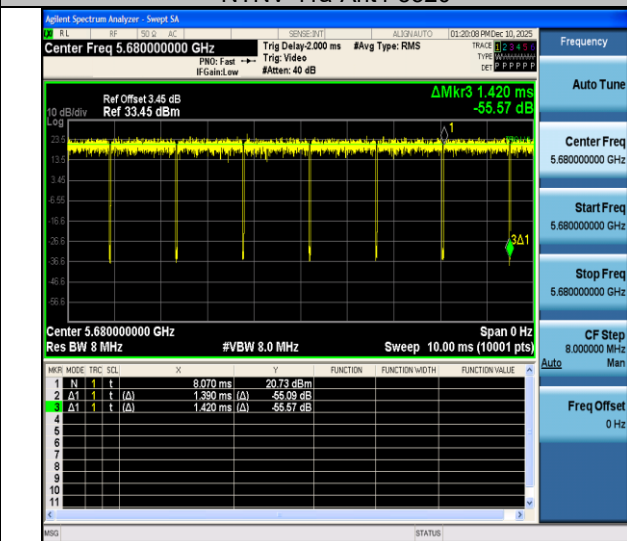
NTNV-11a-Ant4-5680
