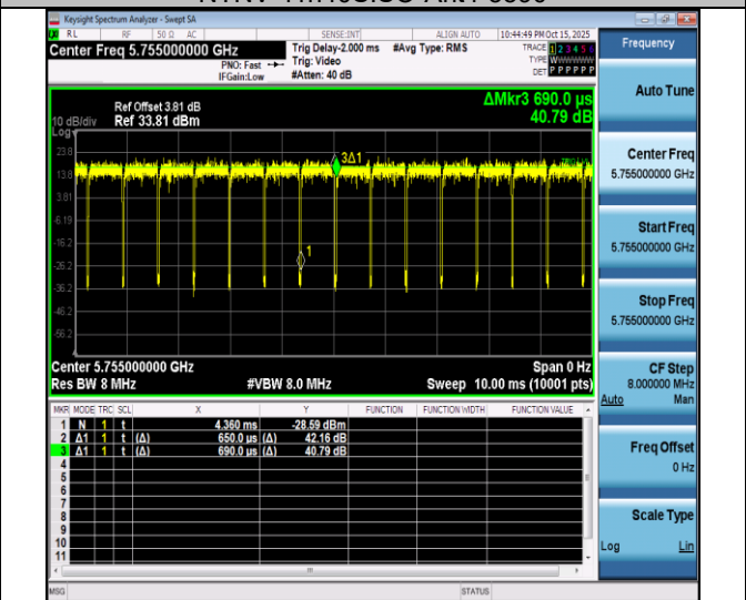
NTNV-11n40SISO-Ant4-5755
