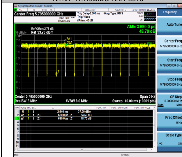
NTNV-11n40SISO-Ant4-5795
