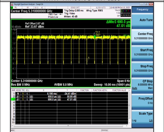
NTNV-11n40SISO-Ant4-5310
