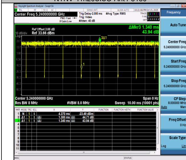
NTNV-11n20SISO-Ant4-5240
