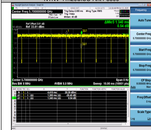
NTNV-11n20SISO-Ant4-5700
