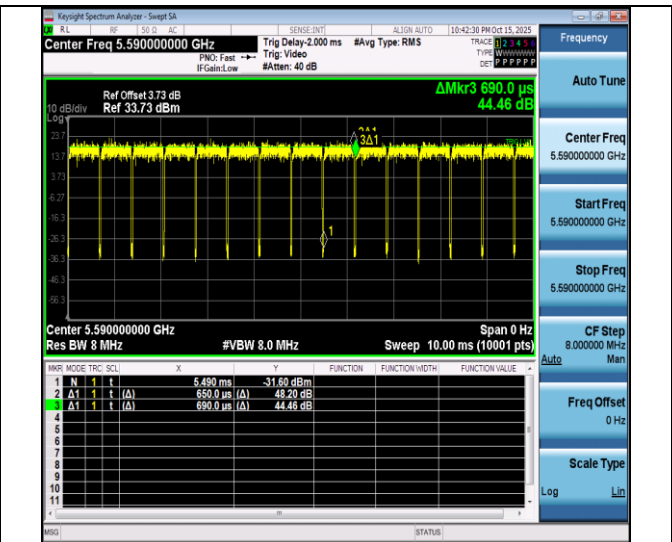
NTNV-11n40SISO-Ant4-5590
