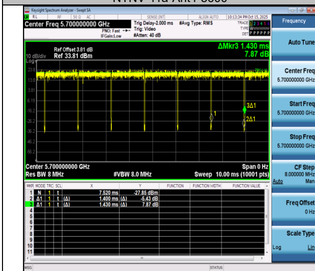
NTNV-11a-Ant4-5700
