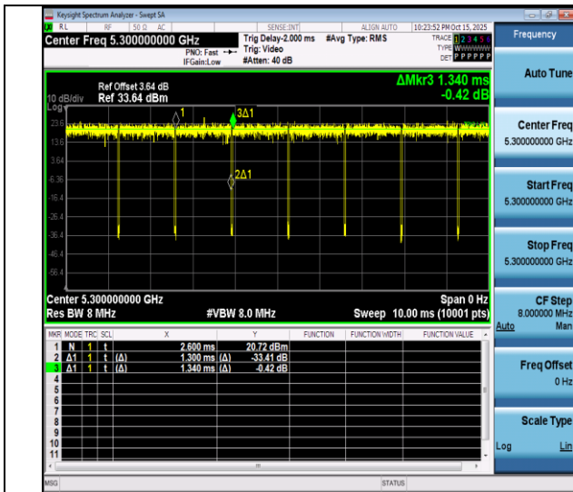
NTNV-11n20SISO-Ant4-5300
