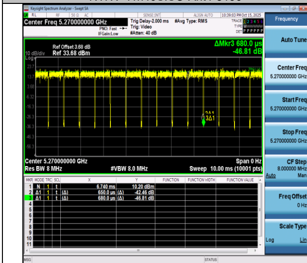
NTNV-11n40SISO-Ant4-5270
