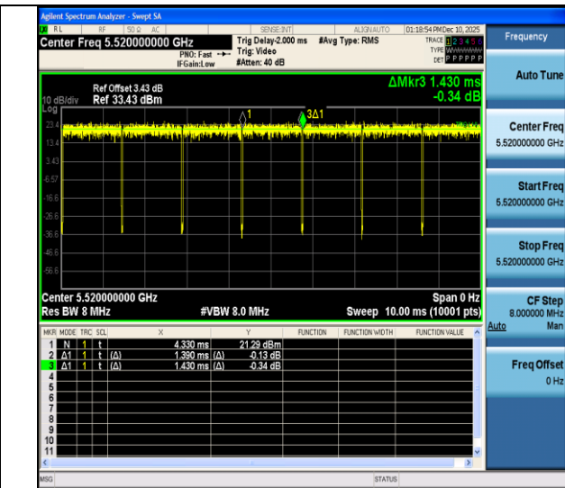
NTNV-11a-Ant4-5520
