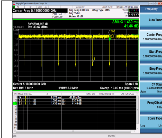
NTNV-11a-Ant4-5180
