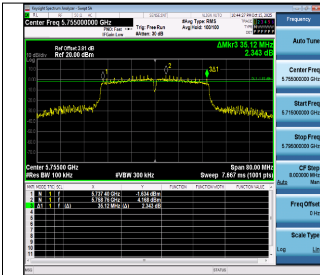
11n40SISO-Ant4-5755-PASS
