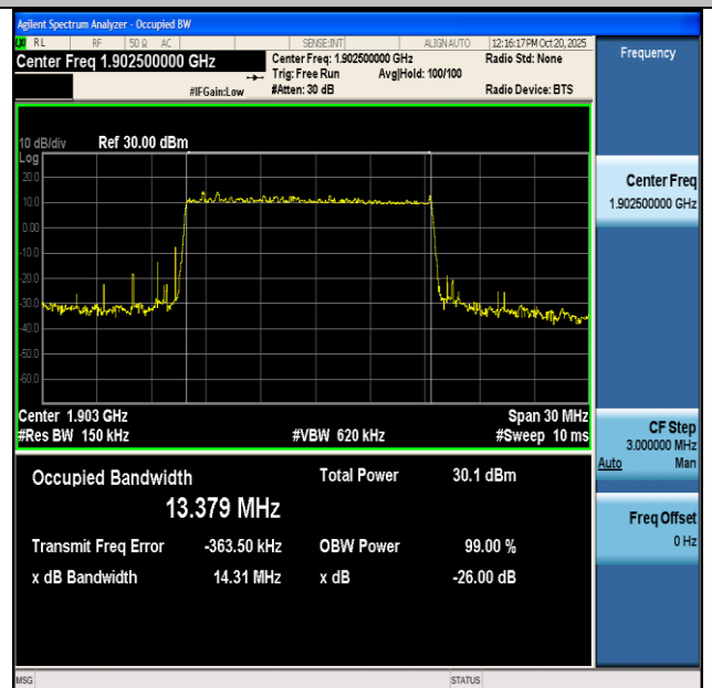
NTNV-n2-PC3-15-15-H-DFT-64QAM-Outer_Full-Ant0-PASS
