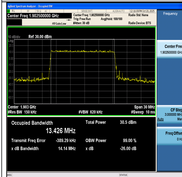
NTNV-n2-PC3-15-15-H-DFT-16QAM-Outer_Full-Ant0-PASS
