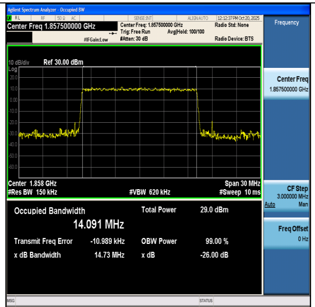
NTNV-n2-PC3-15-15-L-CP-64QAM-Outer_Full-Ant0-PASS
