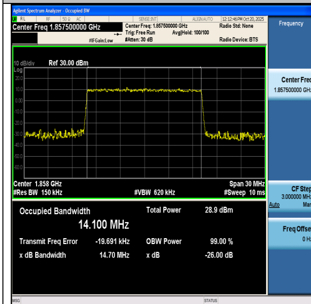
NTNV-n2-PC3-15-15-L-CP-256QAM-Outer_Full-Ant0-PASS
