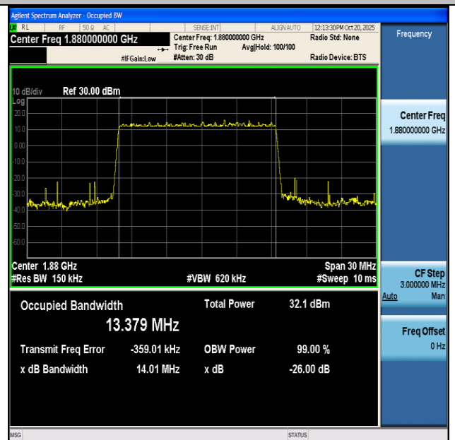
NTNV-n2-PC3-15-15-M-DFT-BPSK-Outer_Full-Ant0-PASS
