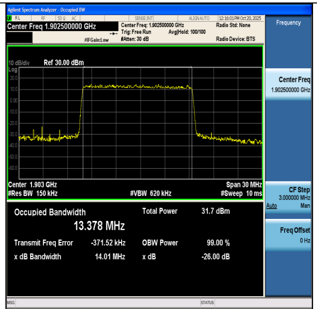
NTNV-n2-PC3-15-15-H-DFT-QPSK-Outer_Full-Ant0-PASS
