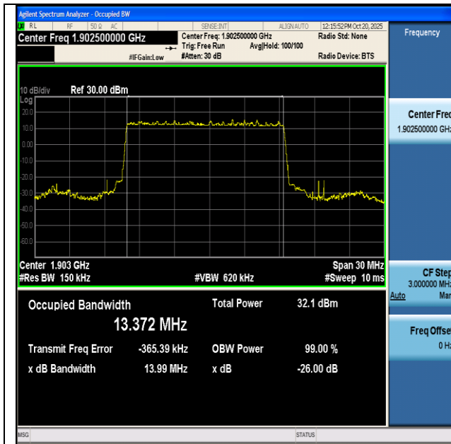
NTNV-n2-PC3-15-15-H-DFT-BPSK-Outer_Full-Ant0-PASS
