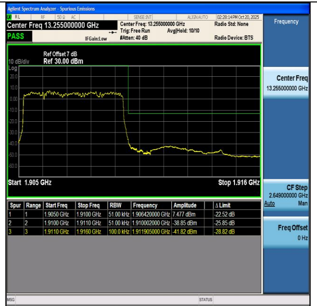
NTNV-n2-PC3-15-5-H-DFT-BPSK-Outer_Full-PASS
