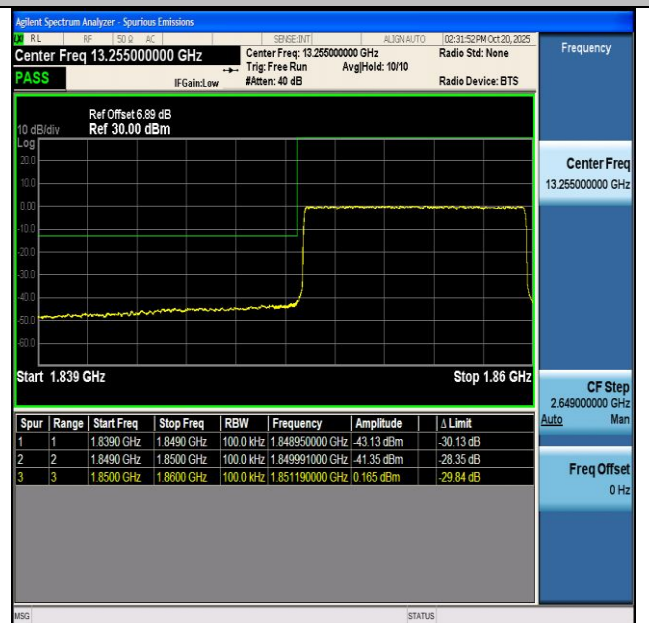
NTNV-n2-PC3-15-10-L-CP-QPSK-Outer_Full-PASS
