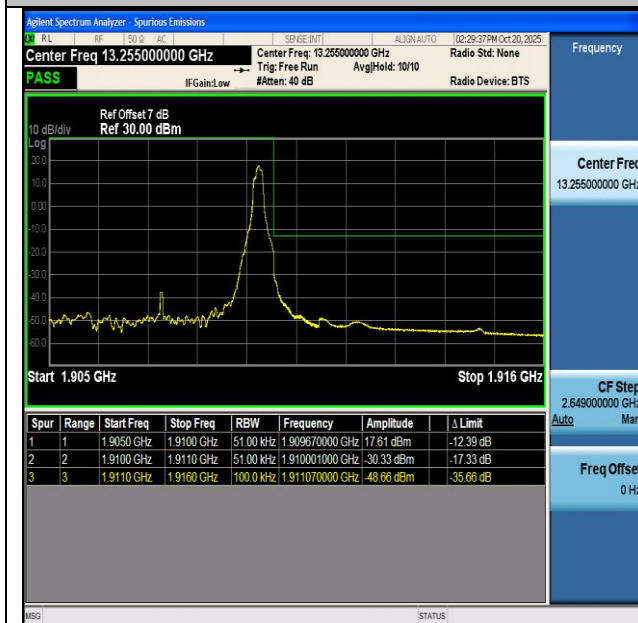
NTNV-n2-PC3-15-5-H-CP-QPSK-Edge_1RB_Right-PASS
