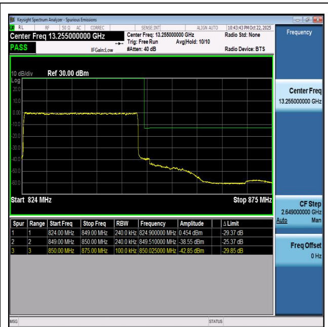
NTNV-n5-PC3-15-25-H-DFT-BPSK-Outer_Full-PASS
