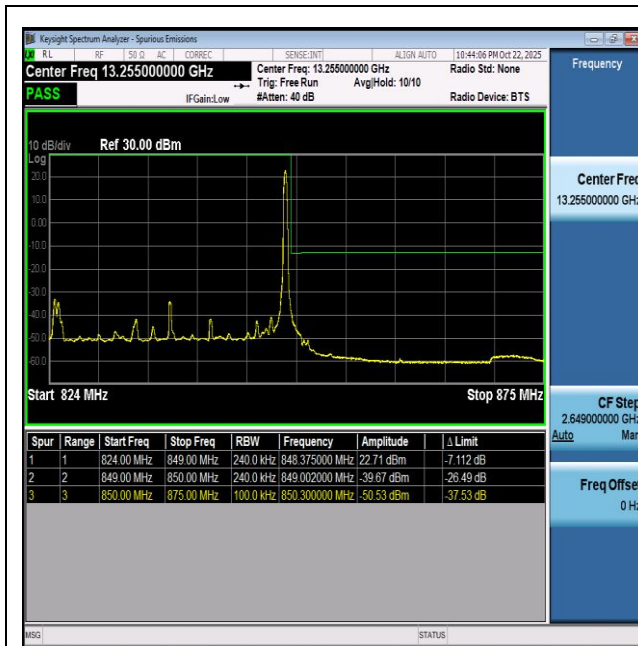
NTNV-n5-PC3-15-25-H-DFT-BPSK-Edge_1RB_Right-PASS
