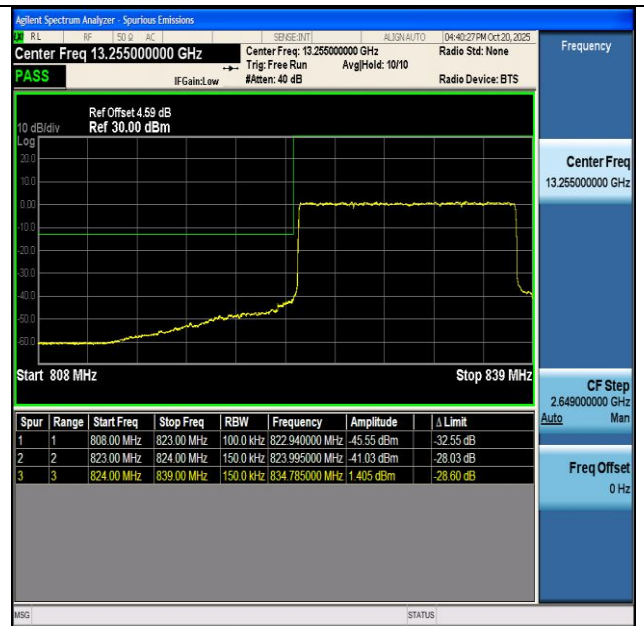
NTNV-n5-PC3-15-15-L-DFT-BPSK-Outer_Full-PASS
