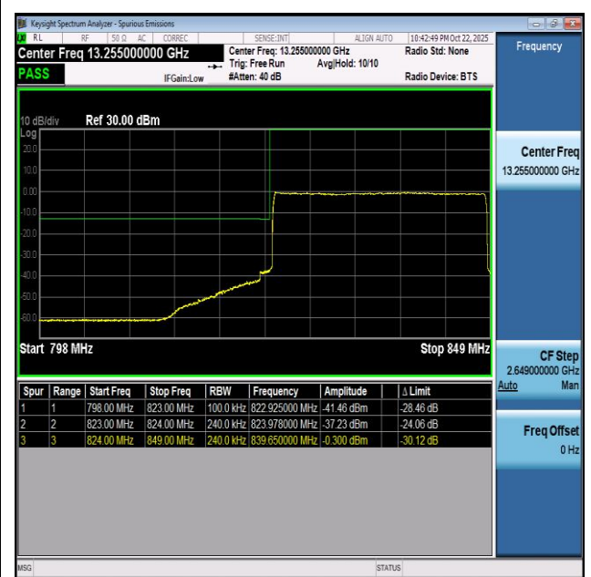
NTVN-n5-PC3-15-25-L-CP-QPSK-Outer_Full-PASS
