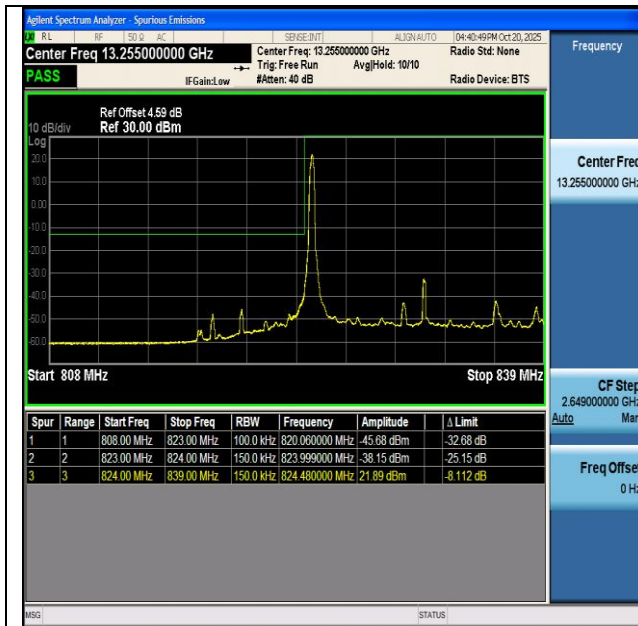
NTNV-n5-PC3-15-15-L-DFT-BPSK-Edge_1RB_Left-PASS
