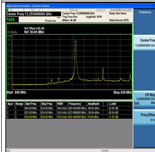
NTNV-n5-PC3-15-15-L-CP-QPSK-Edge_1RB_Left-PASS
