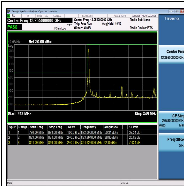
NTVN-n5-PC3-15-25-L-DFT-BPSK-Edge_1RB_Left-PASS
