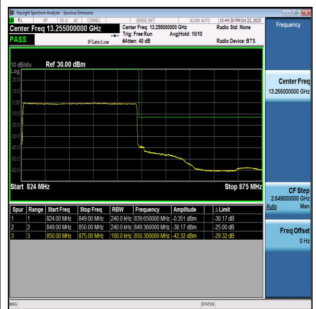
NTNV-n5-PC3-15-25-H-CP-QPSK-Outer_Full-PASS
