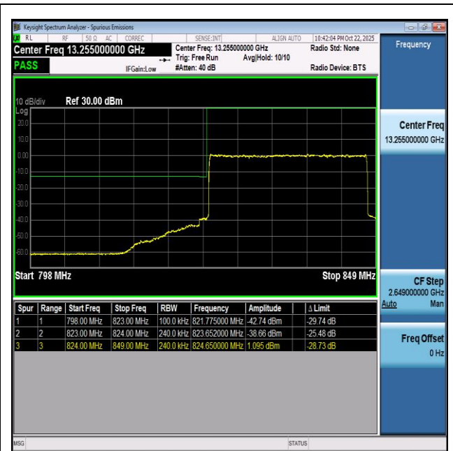
NTVN-n5-PC3-15-25-L-DFT-BPSK-Outer_Full-PASS
