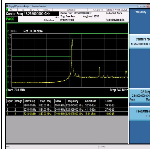
NTVN-n5-PC3-15-25-L-CP-QPSK-Edge_1RB_Left-PASS
