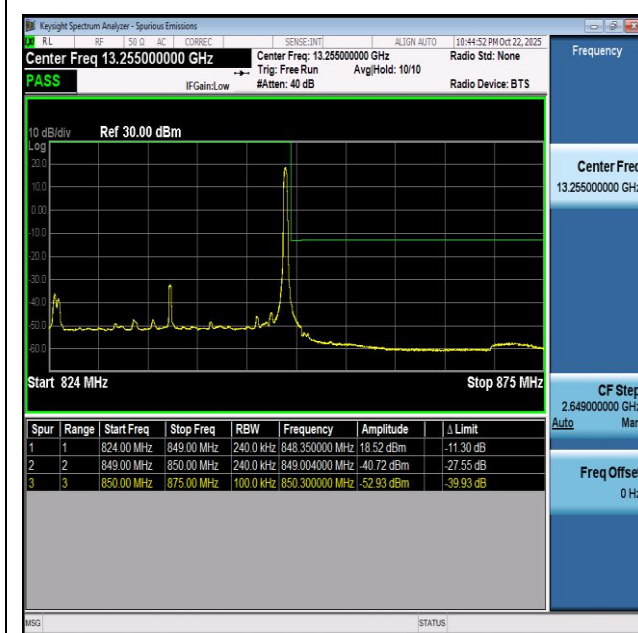
NTNV-n5-PC3-15-25-H-CP-QPSK-Edge_1RB_Right-PASS
