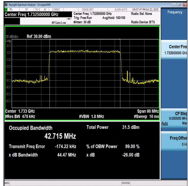
NTNV-n66-PC3-15-45-L-DFT-QPSK-Outer_Full-Ant0-PASS
