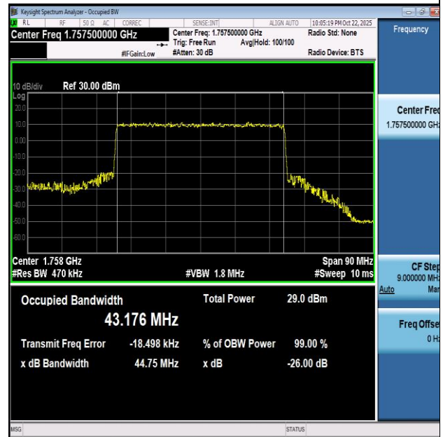
NTNV-n66-PC3-15-45-H-CP-64QAM-Outer_Full-Ant0-PASS
