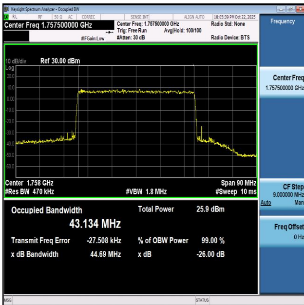
NTNV-n66-PC3-15-45-H-CP-256QAM-Outer_Full-Ant0-PASS
