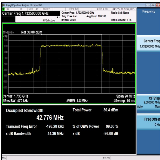
NTNV-n66-PC3-15-45-L-DFT-16QAM-Outer_Full-Ant0-PASS
