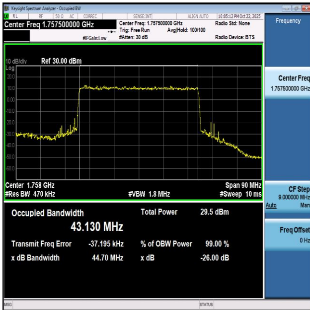
NTNV-n66-PC3-15-45-H-CP-16QAM-Outer_Full-Ant0-PASS
