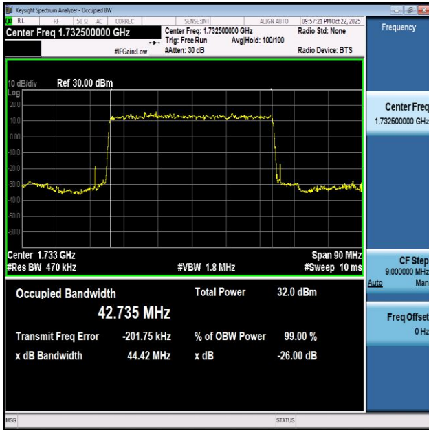
NTNV-n66-PC3-15-45-L-DFT-BPSK-Outer_Full-Ant0-PASS
