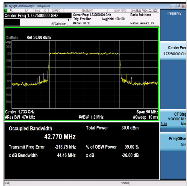
NTNV-n66-PC3-15-45-L-DFT-64QAM-Outer_Full-Ant0-PASS
