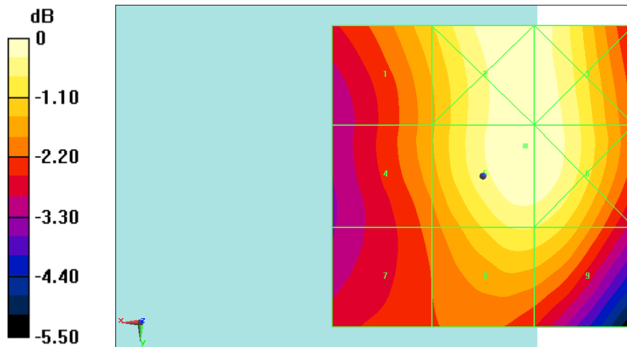
Fig B.1 HAC RF E-Field GSM 850 Mid
