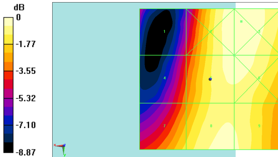
Fig B.2 HAC RF E-Field GSM 1900 Mid
