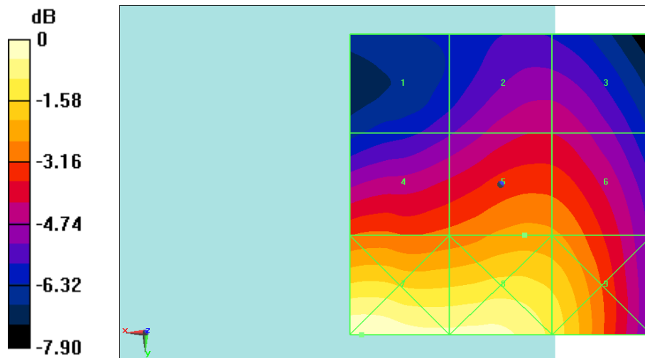
Fig B.3 HAC RF E-Field WiFi2.4G 6M
