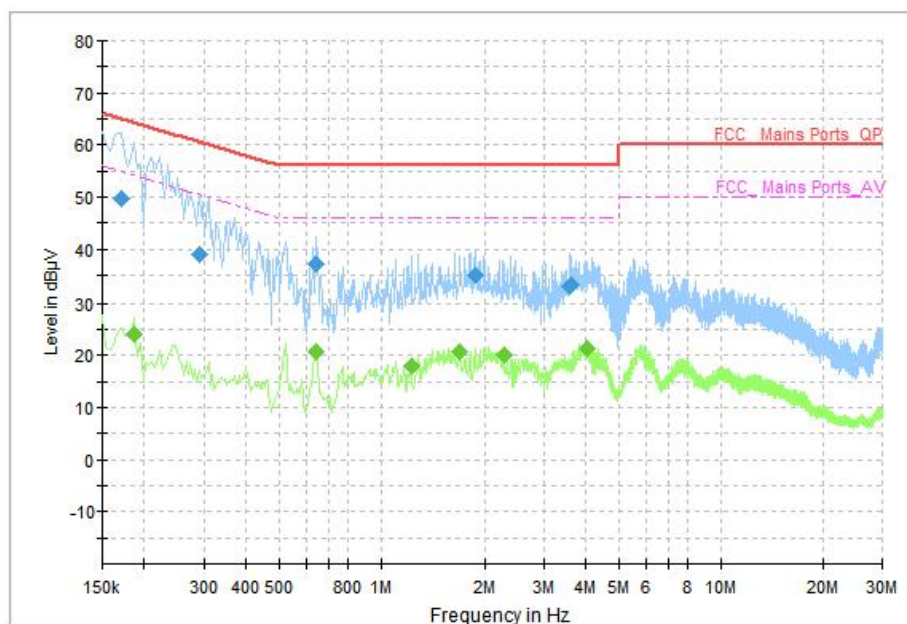
Fig.52 AC Power line Conducted Emission (Idle), LE 1M
