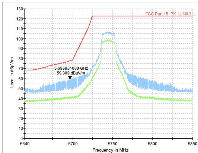
Fig. 67 Band Edges (802.11a, CH149 5745MHz)
