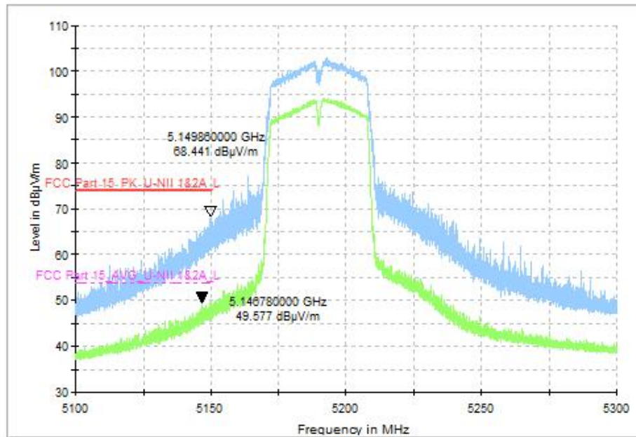
Fig. 69 Band Edges (802.11ac-VHT40, CH38 5190MHz)
