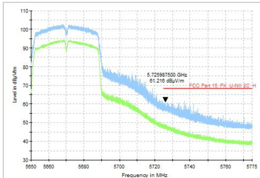
Fig. 72 Band Edges (802.11ac-VHT40, CH134 5670MHz)
