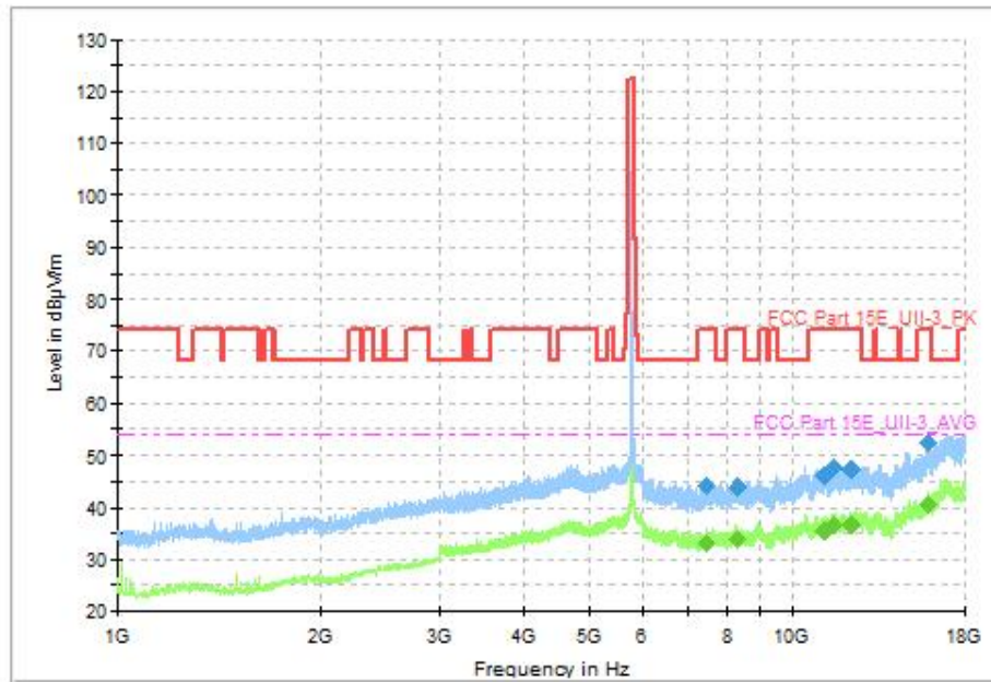
Fig. 90 Transmitter Spurious Emission (802.11a, CH157 5785MHz, 1 GHz-18 GHz)
