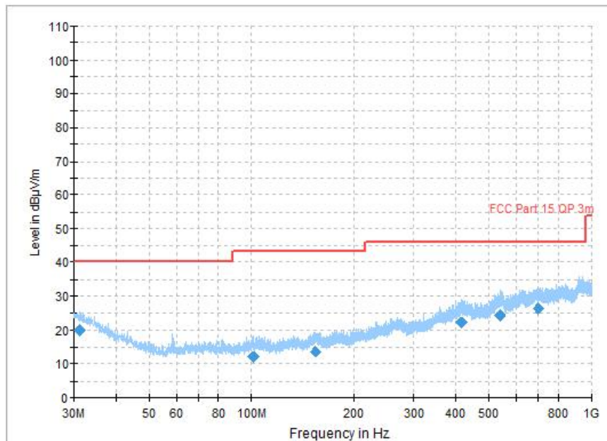
Fig. 106 Transmitter Spurious Emission (All channel, 30MHz~1GHz)
