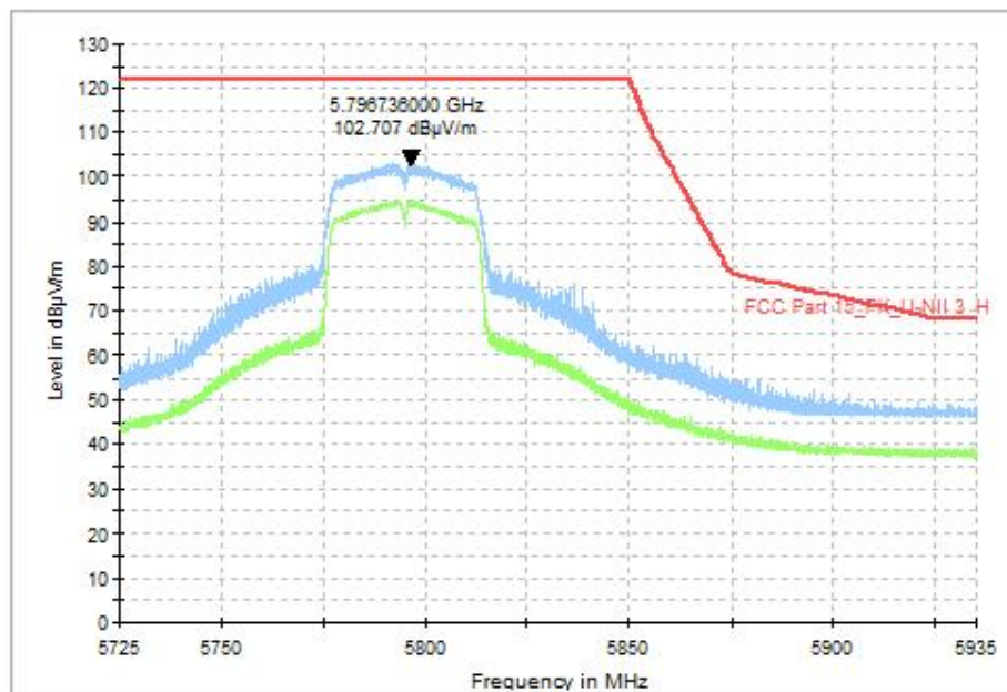
Fig. 74 Band Edges (802.11ac-VHT40, CH159 5795MHz)
