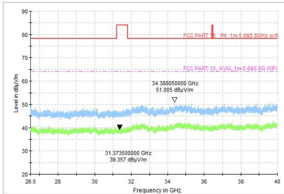
Fig. 108 Transmitter Spurious Emission (All channel, 26.5GHz~40GHz)
