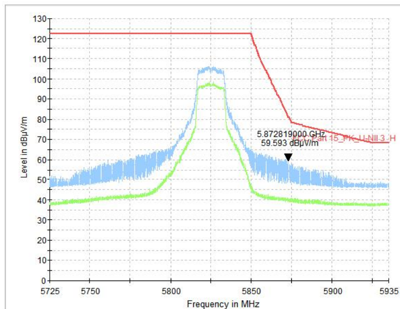
Fig. 68 Band Edges (802.11a, CH165 5825MHz)
