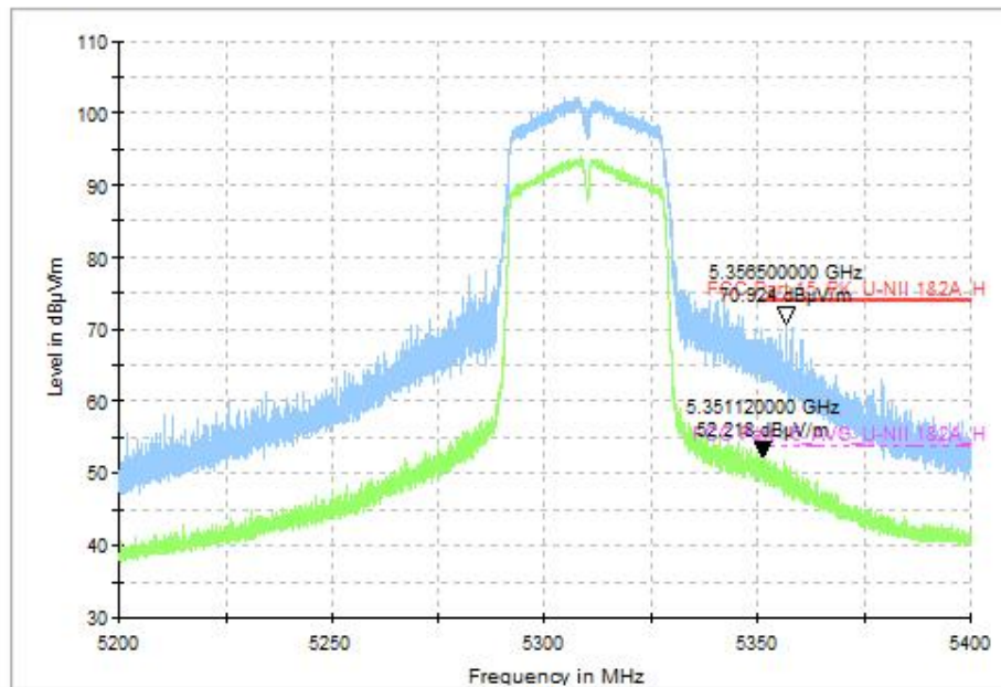
Fig. 70 Band Edges (802.11ac-VHT40, CH62 5310MHz)
