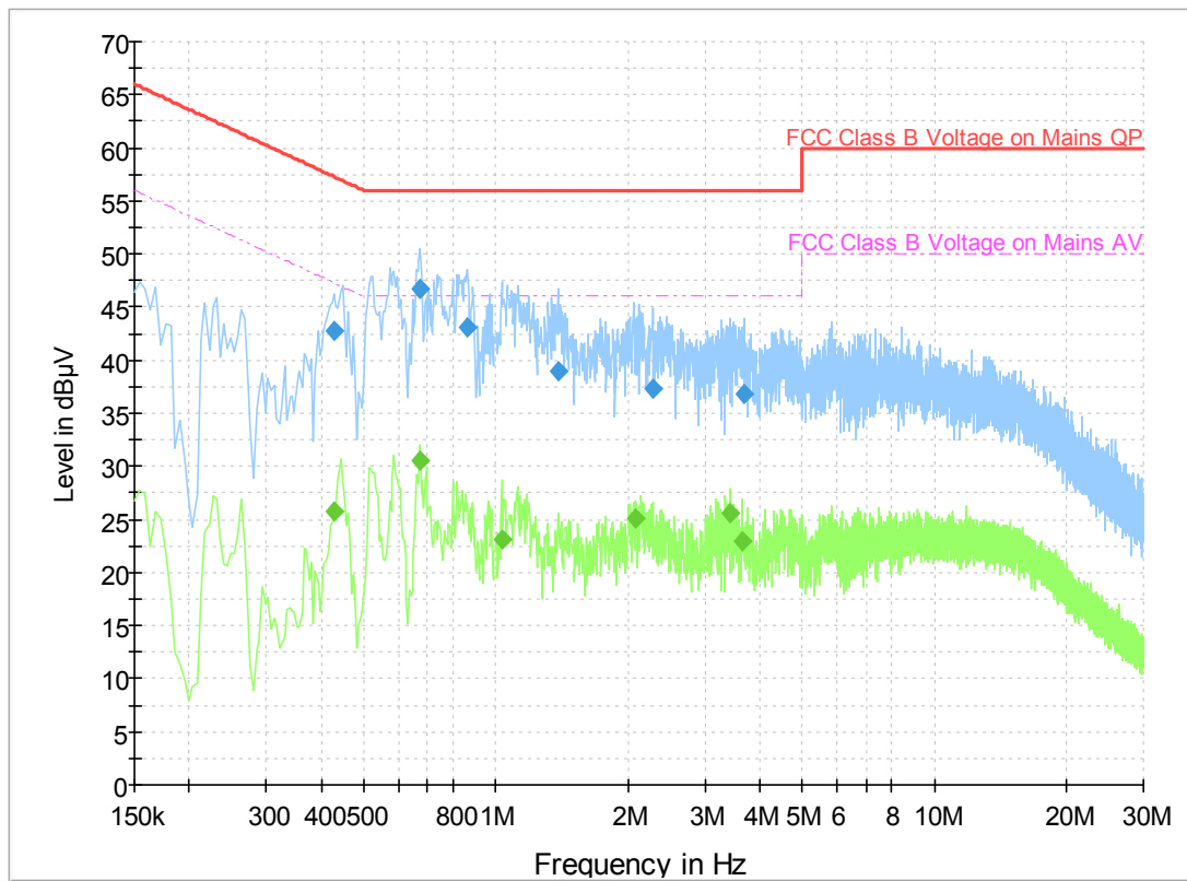
Figure A.10 Conducted Emission
