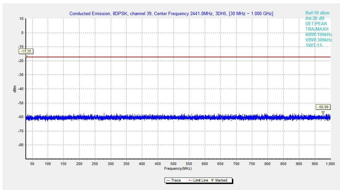
Fig.55. Conducted spurious emission: 8DPSK, Channel 39, 30MHz - 1GHz
