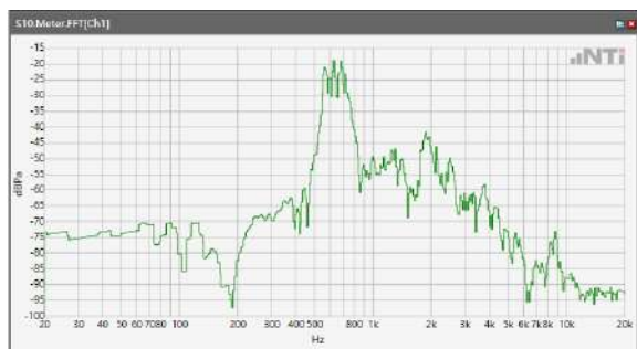
ANSI/TIA 5050-2018 \ 2N HAC OFF \ NB 12.2kbps\ 5.2 Receive path – distortion and noise\ LTE Band 5
