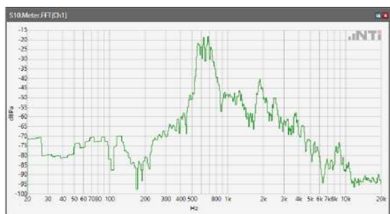
ANSI/TIA 5050-2018 \ 2N HAC OFF \ NB 12.2kbps\ 5.2 Receive path – distortion and noise\ LTE Band 12
