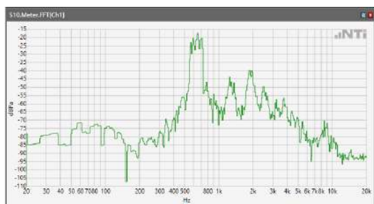
ANSI/TIA 5050-2018 \ 2N HAC OFF \ NB 12.2kbps\ 5.2 Receive path – distortion and noise\ LTE Band 14
