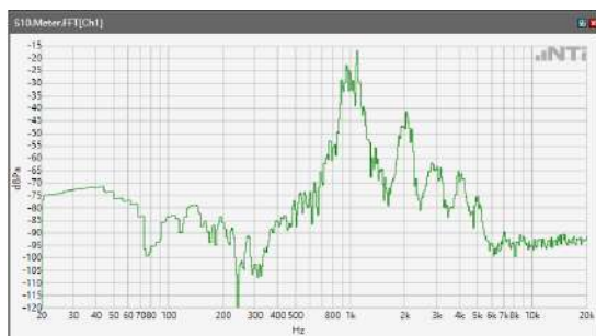
ANSI/TIA 5050-2018 \ 2N HAC OFF \ NB 12.2kbps\ 5.2 Receive path – distortion and noise\ 5GNR n71
