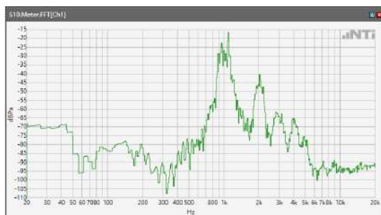
ANSI/TIA 5050-2018 \ 2N HAC OFF \ NB 12.2kbps\ 5.2 Receive path – distortion and noise\ 5GNR n77
