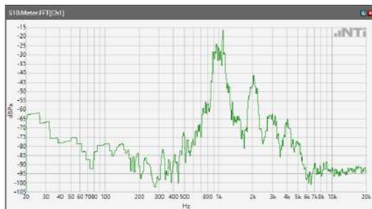
ANSI/TIA 5050-2018 \ 2N HAC OFF \ NB 12.2kbps\ 5.2 Receive path – distortion and noise\ WLAN2.4G
