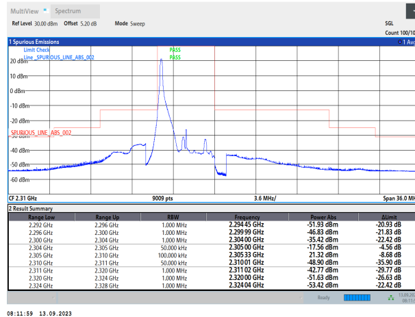
Band30-5MHz-QPSK-27685-25RB#0
