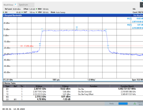
Band30-5MHz-16QAM-27710-25RB#0
