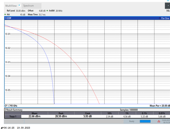
Band66-20MHz-QPSK-132322-100RB#0
