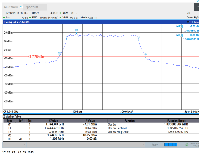
Band66-1.4MHz-16QAM-132322-6RB#0
