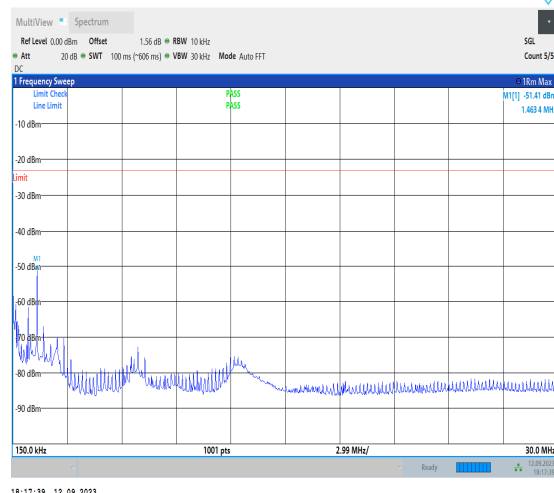
1-N71-PC3-15-20-H-1-DFT-PI2BPSK-Inner_1RB_L t-1@1-0.15-30-Ant1-1.46--51.41--23-PASS
