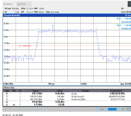
1-N71-PC3-15-5-M-4-DFT-64QAM-Outer_Full-25@0- -Ant1-4.46-4.750-≤5-PASS
