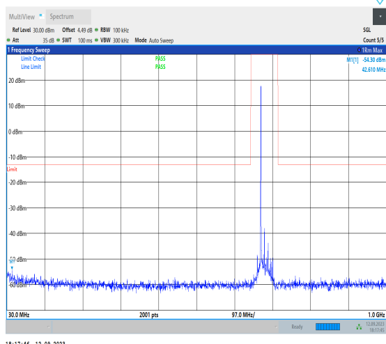
1-N71-PC3-15-20-H-1-DFT-PI2BPSK-Inner_1RB_L eft-1@1-30-1000-Ant1-42.61--54.30--13-PASS
