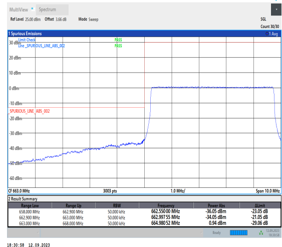
1-N71-PC3-15-5-L-6-CP-QPSK-Outer_Full-25@0-Ant1-1--PASS-see graph
