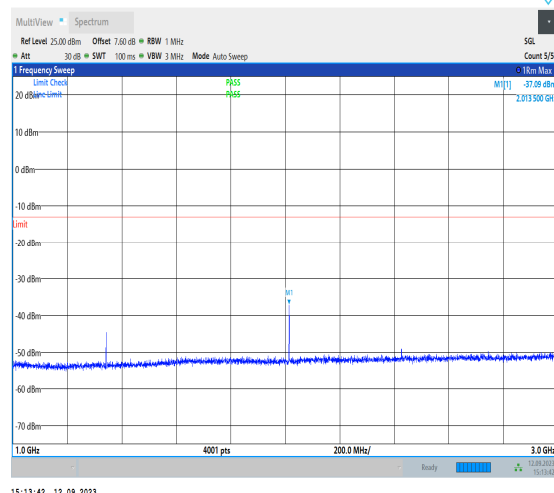
1-N71-PC3-15-20-M-1-DFT-PI2BPSK-Inner_1RB_Lef t-1@1-1000-3000-Ant1-2013.50--37.09--13-PASS
