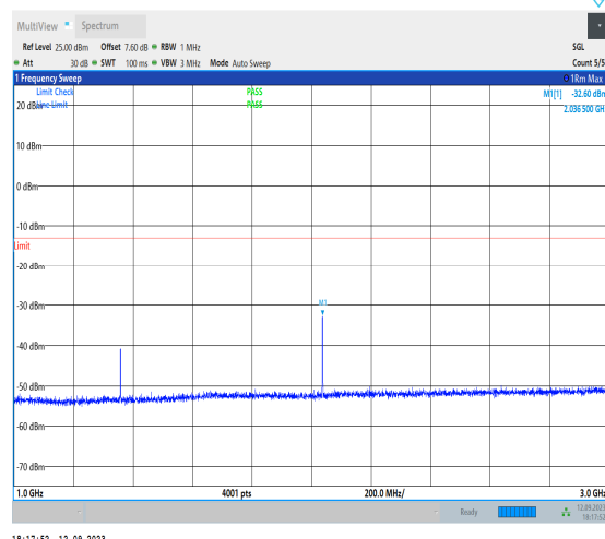
1-N71-PC3-15-20-H-1-DFT-PI2BPSK-Inner_1RB_L t-1@1-1000-3000-Ant1-2036.50--32.60--13-PASS
