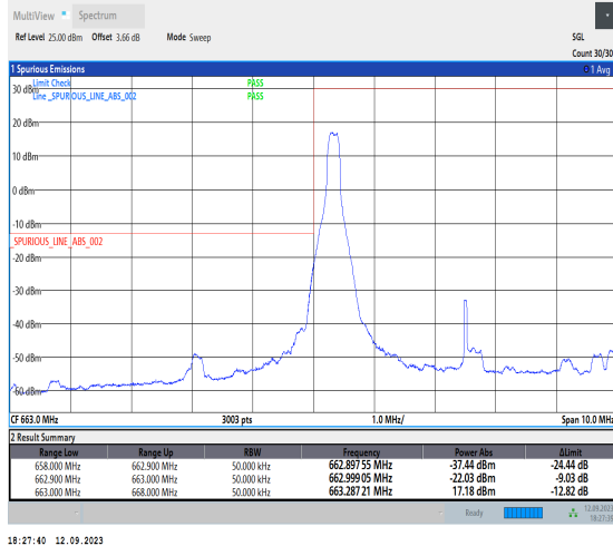
1-N71-PC3-15-5-L-1-DFT-PI2BPSK-Edge_1RB_Left-1 @0-Ant1-1--PASS-see graph
