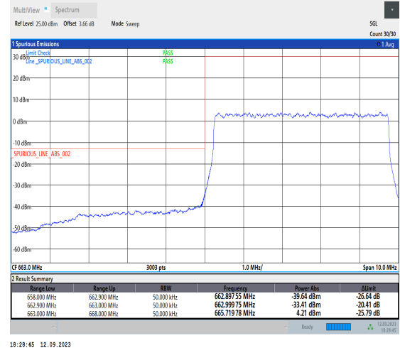
1-N71-PC3-15-5-L-3-DFT-PI2BPSK-Outer_Full-25 @0-Ant1-1--PASS-see graph
