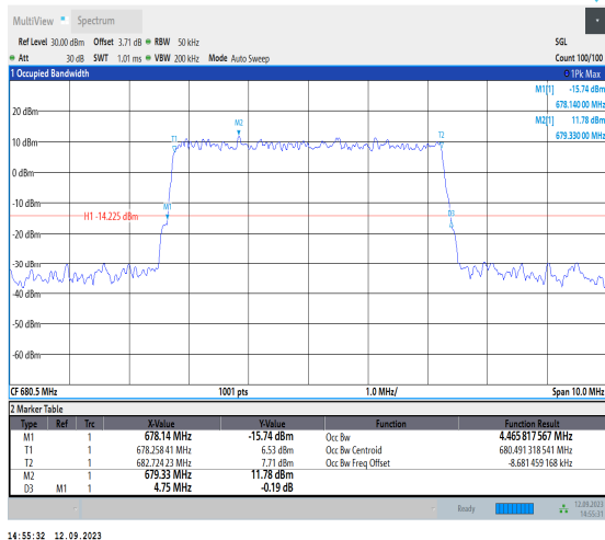
1-N71-PC3-15-5-M-1-DFT-QPSK-Outer_Full-25@0- Ant1-4.466-4.750-≤5-PASS
