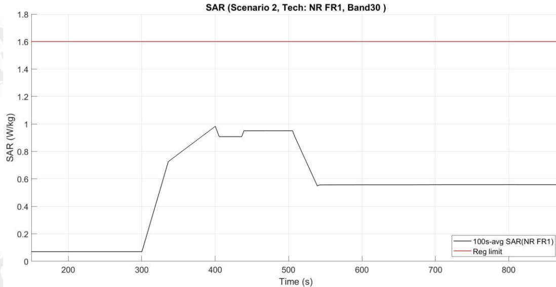
Figure 5- 9 Time-averaged SAR for case 3 (sub6 NR n30)
