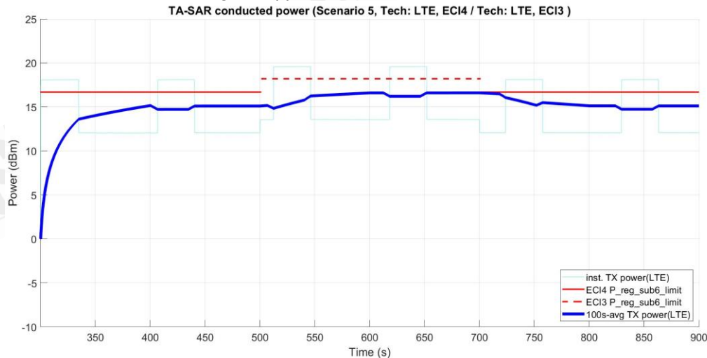
Figure 5- 28 Time-averaged conducted TX power over time for case 11 (LTE Band 30)
