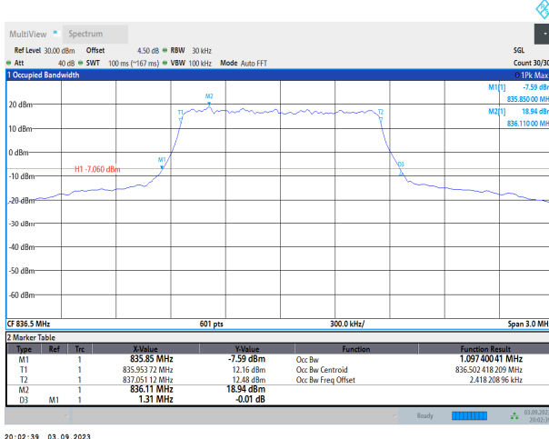
Band26-1.4MHz-16QAM-26915-6RB#0
