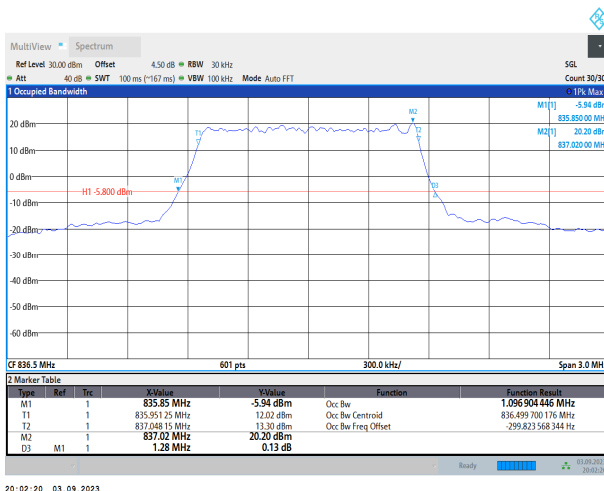
Band26-1.4MHz-16QAM-26915-6RB#0
