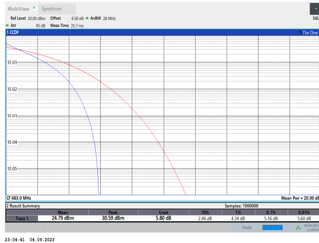
Band71-20MHz-QPSK-133322-100RB#0
