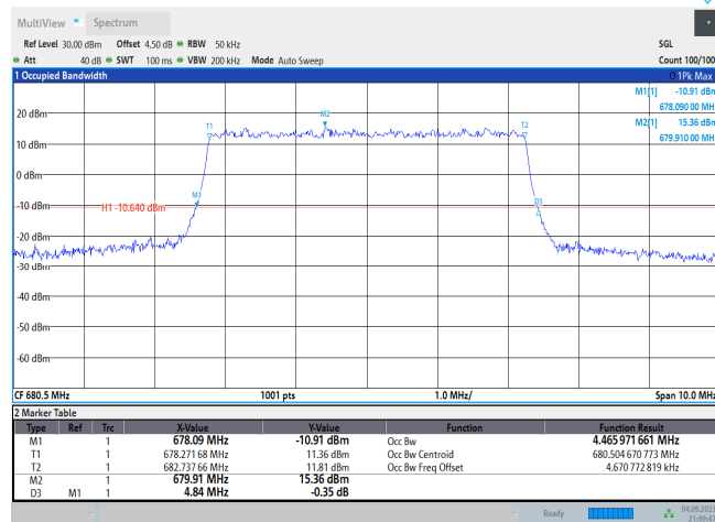
Band71-5MHz-16QAM-133297-25RB#0
