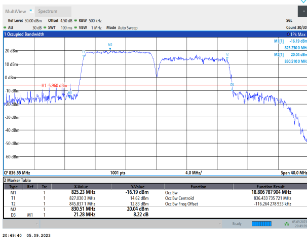
5-5-10MHz-10MHz-16QAM-16QAM-20476-20575-50RB#0-50RB#0
