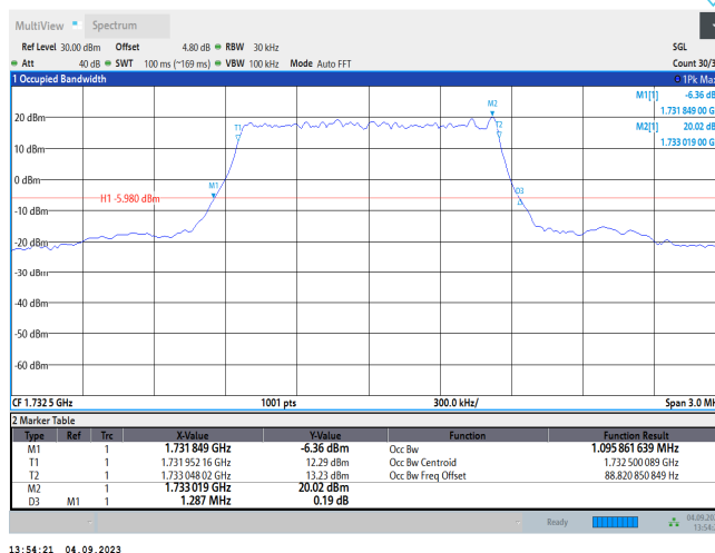
Band4-1.4MHz-16QAM-20175-6RB#0
