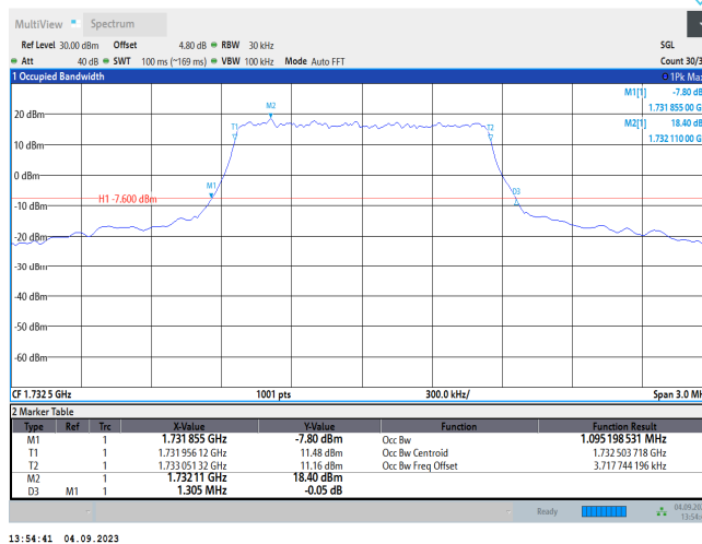
Band4-1.4MHz-16QAM-20175-6RB#0
