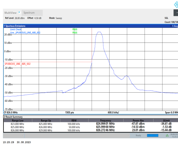
Band5-1.4MHz-QPSK-20427-6RB#0
