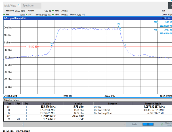
Band5-1.4MHz-16QAM-20525-6RB#0
