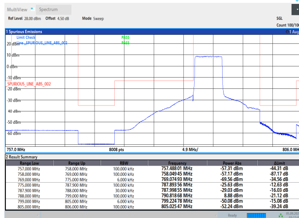
Band14-5MHz-QPSK-23305-25RB#0
