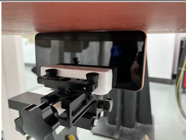
Photo 22: Left Side 0mm for NFC
