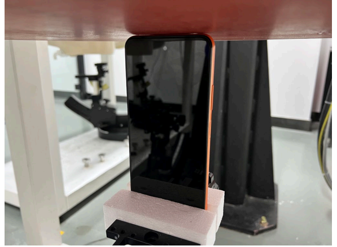
Photo 25: Top Side 0mm for NFC
