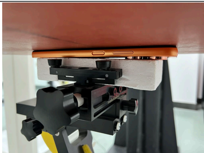
Photo 23: Right Side 0mm for NFC
