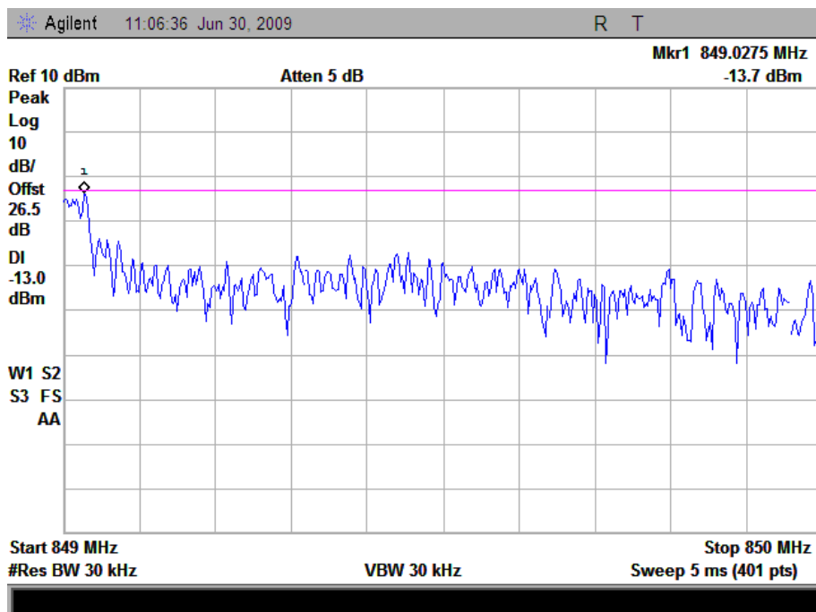
(Plot B: CDMA 800MHz Channel = 777)
