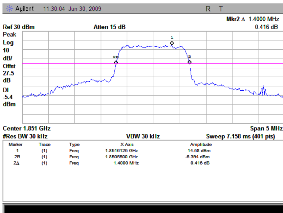
(Plot D: CDMA 1900MHz Channel = 25)
