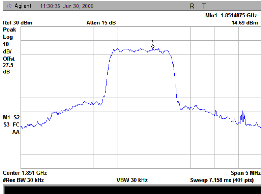
(Plot C: CDMA 1900MHz Channel = 25)
