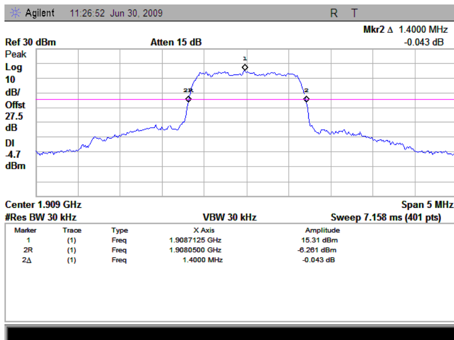
(Plot F: CDMA 1900MHz Channel = 1175)
