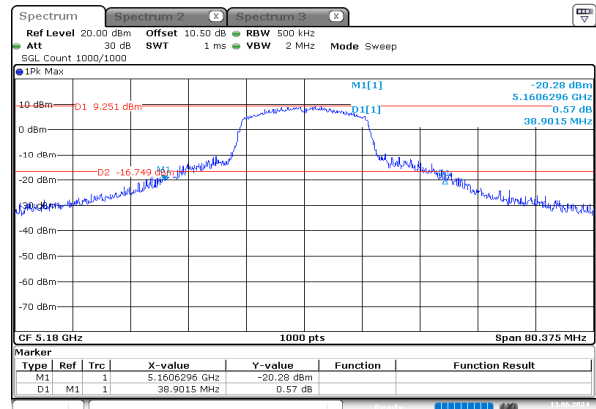
n20_5180MHz_Chain 0
