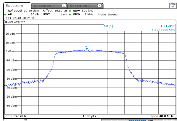
a_5825MHz_Chain 0
