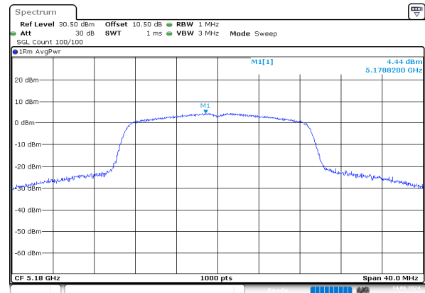
n20_5180MHz_Chain 0
