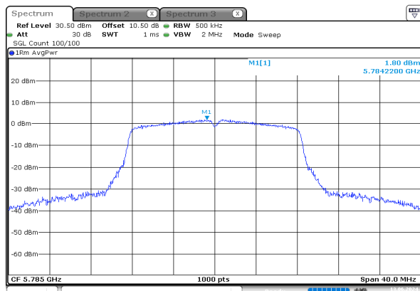
a_5785MHz_Chain 0
