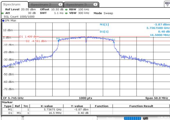
a_5745MHz_Chain 0
