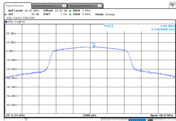
n20_5240MHz_Chain 0
