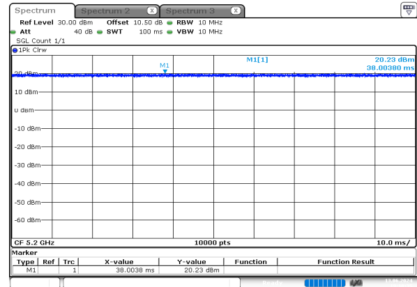
n20_5200MHz_Chain 0
