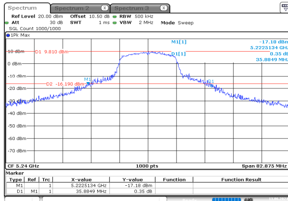
a_5240MHz_Chain 0
