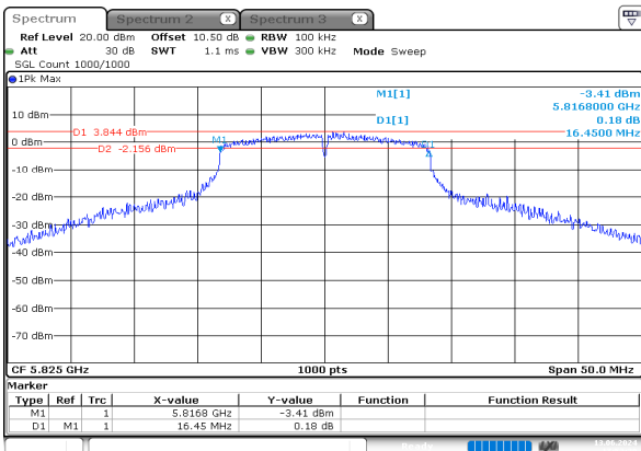
a_5825MHz_Chain 0
