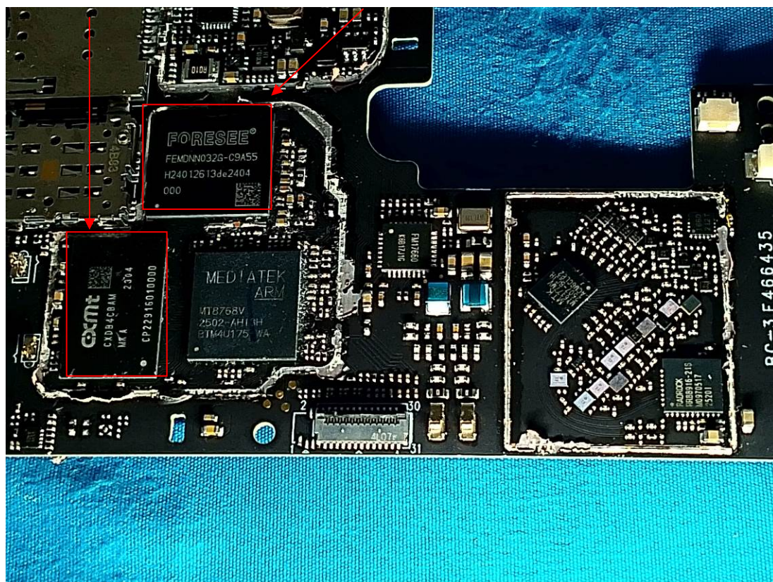
Memory(2GB)
