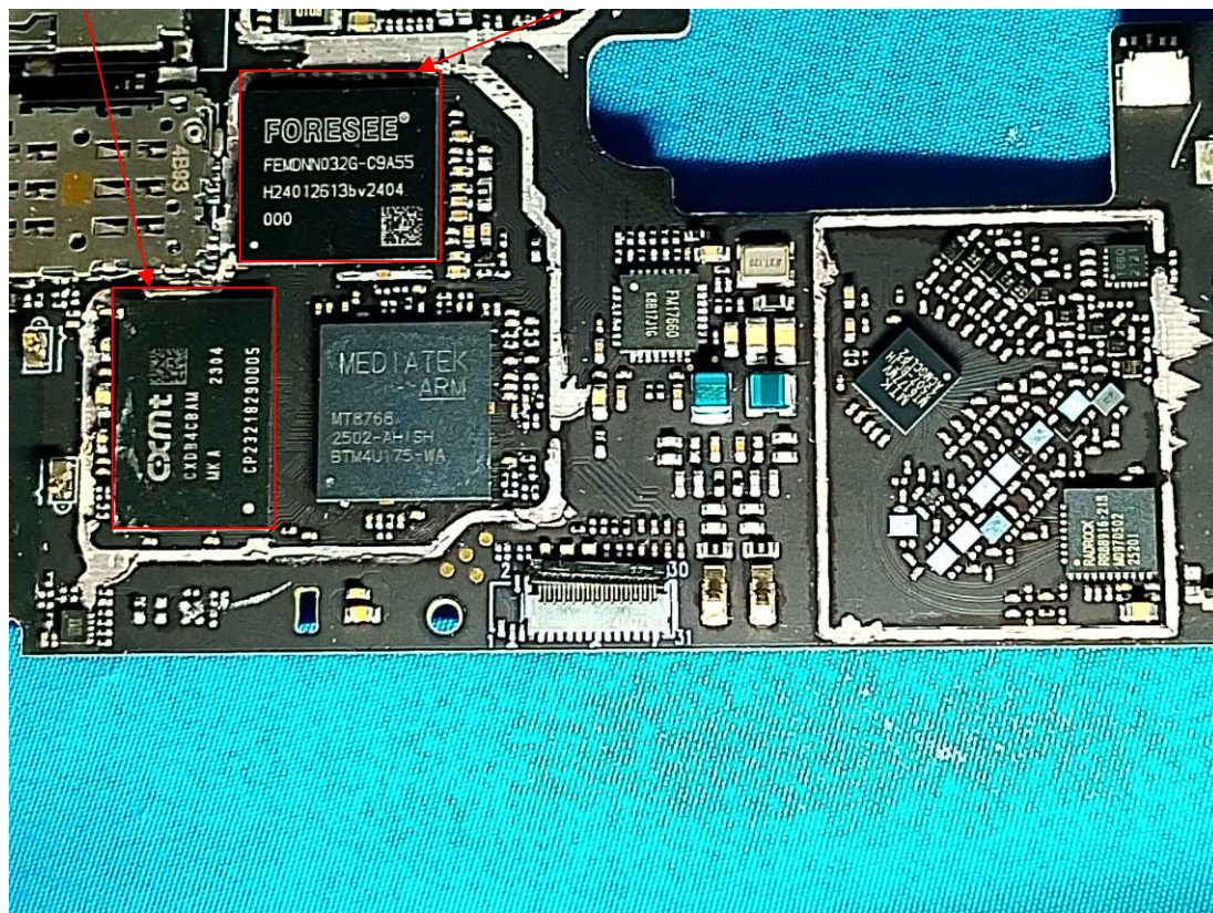
Memory(2GB)
