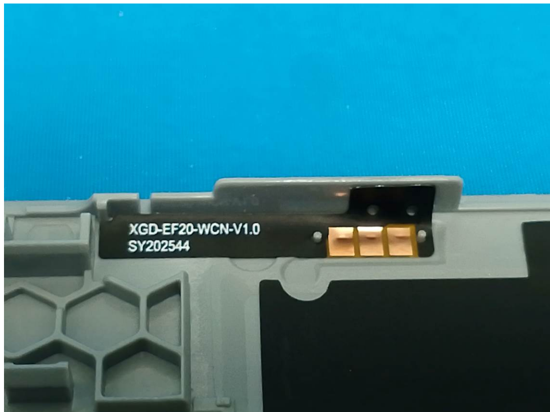
Bluetooth&Wifi Antenna(ANT 2)
