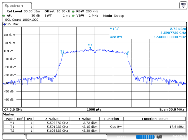
802.11n20_5600MHz
